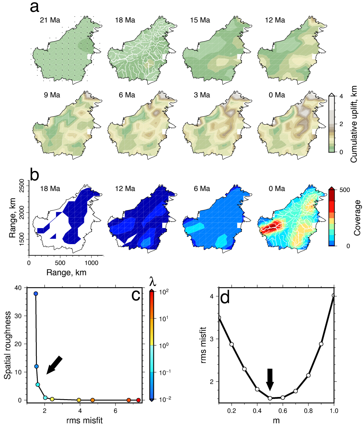
Figure 6: (a) Calculated cumulative uplift history of Borneo. Solid circles = vertices at which uplift rate is calculated during inverse modeling. White lines = recovered drainage network used for inverse modeling. (b) Model coverage (nullity) plots showing number of non-zero entries in model matrix. (c) Residual rms misfit plotted as function of spatial smoothing, \lambda . Black arrow = locus of smoothest model that yields minimum misfit. (d) Residual rms misfit plotted as function of m . Black arrow = locus of global minimum at m = 0.5 .
