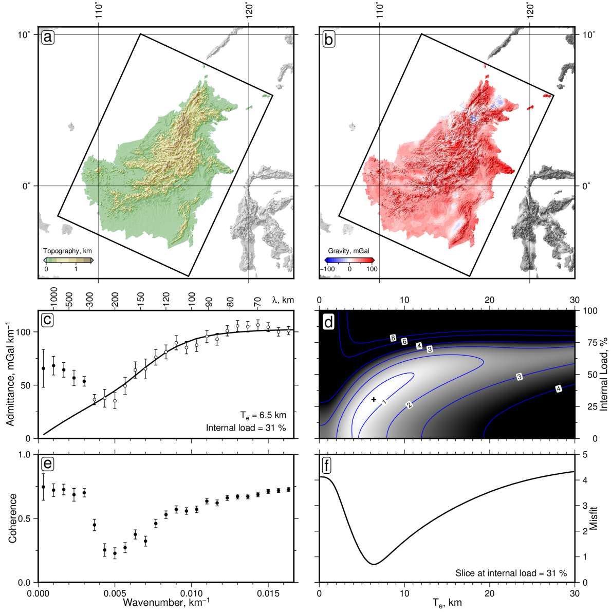
Figure 3: (a) Topographic map of Borneo determined using SRTM_30_plus database ( Becker et al. , 2009). Box = region for which admittance analysis was carried out. (b) Free-air gravity map of Borneo determined using Eigen-6C_3stat database ( Forste et al. , 2012). (c) Admittance plotted as function of wavenumber. Open/solid circles with error bars = values of admittance determined by spectral analysis of topography and gravity; black line = admittance as function of wavenumber that best fits open circles for elastic thickness, T_e = 7 \pm 3 km; crustal thickness = 30 km; upper crustal thickness = 15 km; density of upper/lower crust = 2.45/2.9 Mg m -3 , respectively. (d) Contoured rms misfit between observed and calculated admittance as function of elastic thickness, T_e , and percentage of internal load. Cross = locus of global minimum. (e) Coherence between topography and gravity as function of wavenumber. (f) Vertical slice through misfit function shown in panel (d) with global minimum at T_e = 7 \pm 3 km for internal load of 31%.
