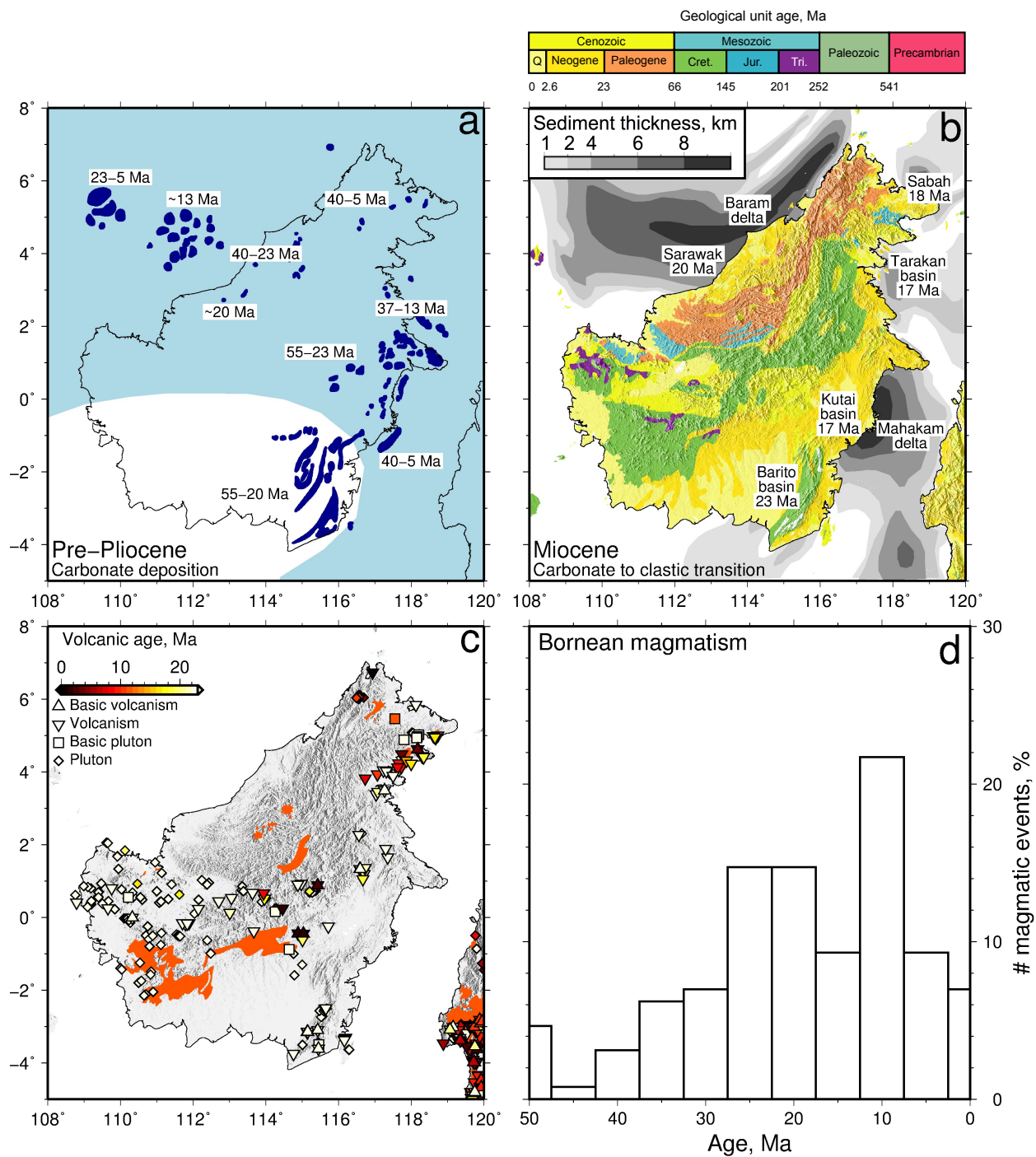
Figure 4: (a) Pre-Pliocene paleogeography of region encompassing Borneo. Dark blue polygons = loci of Cenozoic marine carbonate deposits ( Wilson et al. , 1999). Light blue shading = distribution of Late Eocene marine conditions ( Hall , 2009). (b) Miocene-Recent paleogeography. Colored units and bar = Mesozoic and Cenozoic stratigraphy ( Choubert & Faure-Muret , 1976). Numbered labels = ages of transition from carbonate to clastic deposition ( Wilson & Moss , 1999); gray isopachs = thickness of Cenozoic sedimentary deposits ( Hall & Nichols , 2002). (c) Temporal and spatial distribution of magmatism from SEARG catalog (e.g. Moss et al. , 1998; Macpherson et al. , 2010). Orange polygons = basaltic igneous rocks ( Choubert & Faure-Muret , 1976); triangles/squares/diamonds = intrusive/extrusive igneous rocks as indicated. (d) Histogram of Bornean magmatism taken from SEARG catalogue.
