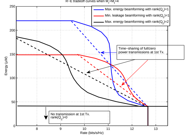
Fig. 3. R-E tradeoff curves for MEBs ( \text{rank}(\mathbf{Q}_1) = \{1, 2\} ) and MLB ( \text{rank}(\mathbf{Q}_1) = 1 ) when M = 4 , \alpha_{ii} = 1 for i = 1, 2 , and \alpha_{ij} = 0.8 for i \neq j .
