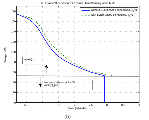
Fig. 8. R-E tradeoff curves for SLER maximizing beamforming with/without SLER-based scheduling when (a) \alpha_{ij} = 0.7 and (b) \alpha_{ij} = 1 for i \neq j . Here, M = 2 .
