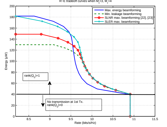
Fig. 7. R-E tradeoff curves for MEB, the MLB, SLNR maximizing beamforming, and SLER maximizing beamforming when M_t = 3 and M_r = 4 .
