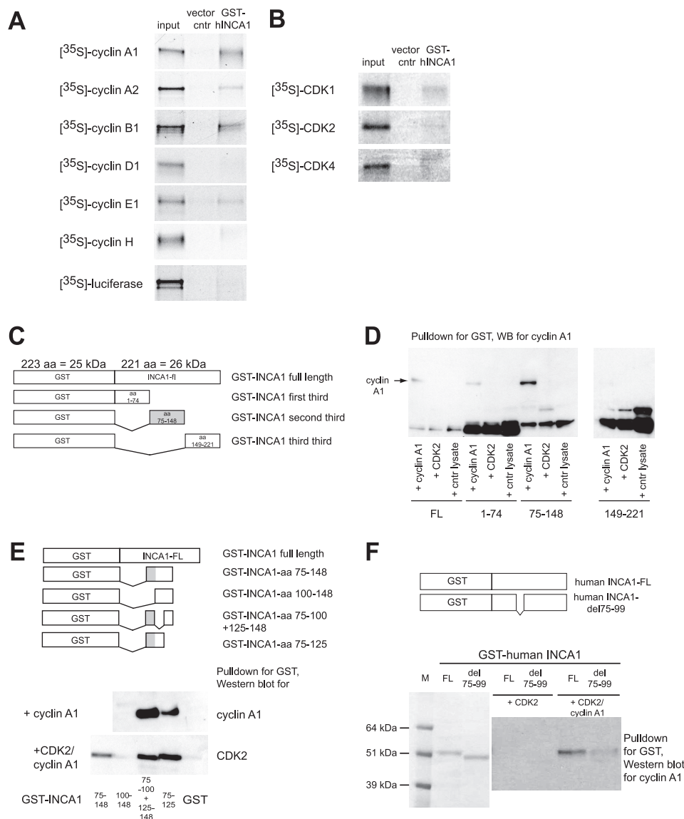
FIGURE 1. GST-pulldown assays revealed a cyclin A1-binding site at amino acids 75–99 in the human INCA1 protein. A , GST pulldown assays using 35 S-labeled cyclins and GST-INCA1 were performed to identify INCA1-binding cyclins. INCA1 interacted directly with the CDK2-specific cyclins A1, A2, B1, and E1 but not with cyclin D1 or H. B , GST pulldown assays as in A revealed only weak binding of GST-INCA1 to CDKs. C , constructs used to determine cyclin-CDK-binding sites in initial experiments. Because the domain structure of INCA1 is unknown, three different deletion mutants were generated and tested. The gray box indicates the binding site. aa, amino acids. D , cyclin A1 bound to amino acids 75–148 of human INCA1. The weak band in this blot at amino acids 1–74 was not consistently reproducible. No binding to amino acids 149–221 was observed. The lower bands are nonspecific. WB, Western blot. E , upper panel, further GST-INCA1 deletions were constructed to localize the region responsible for CDK and cyclin binding. The gray box indicates the binding site. Lower panel, pulldown assays using further deletion mutants indicate that amino acids at positions 75–99 of INCA1 are required and sufficient for binding of cyclin A1 and CDK2. F , amino acids 75–99 that are required for cyclin-CDK binding were deleted in the full-length construct (upper panel). Coomassie staining of the proteins expressed in E. coli from the constructs to determine the equal amounts of both proteins for the pulldown assays depicted (lower panel, left side). Upon incubation with CDK2 and cyclin A1, the INCA1 deletion mutant del75–99 showed strongly decreased binding affinity for cyclin A1 (lower panel, right side). M, marker; FL, full-length INCA1; del 75–99, deletion mutant of full-length INCA1 lacking amino acids 75–99.
