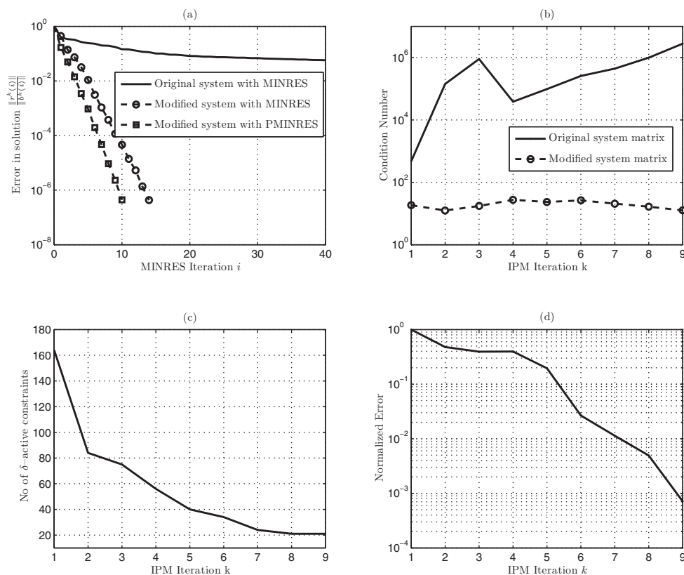
FIG. 6.1. Results for a system with n = 10 , m = 2 , and N = 20 : (a) Comparison of rate of convergence on solving the original linear system (2.10) and approximate linear system (3.8) or (3.9) with MINRES and PMINRES for k = 3 . (b) Comparison of condition numbers of original matrix A_1^k of (2.10a) and modified matrix A_1^k of (3.7a). (c) Decay of number of \delta -active inequality constraints with main loop iteration k . (d) Decay of normalized error \|e^k\|_\infty / \|e^0\|_\infty in the solution of the modified system (3.8), where \|e^k\|_\infty := \|[e_1^k \ e_2^k]\|_\infty . The upper bounds on e_1^k and e_2^k are defined in (3.13).
