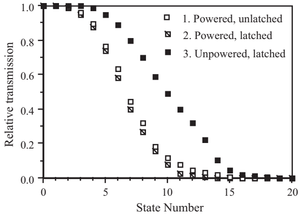
Fig. 6. Measured attenuation achieved when the shutter is 1) powered, but not latched, 2) powered and mechanically latched, and 3) latched, but all drive power is removed.
