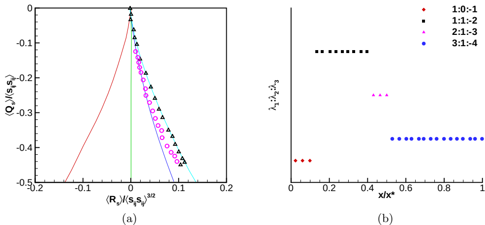
Figure 18: (a) Mean trajectory of Q_s and R_s in the phase map. Triangles represent the production region while circles the decay region. (b) Eigenvalue ratios \lambda_1 : \lambda_2 : \lambda_3 along the grid-element centreline.
