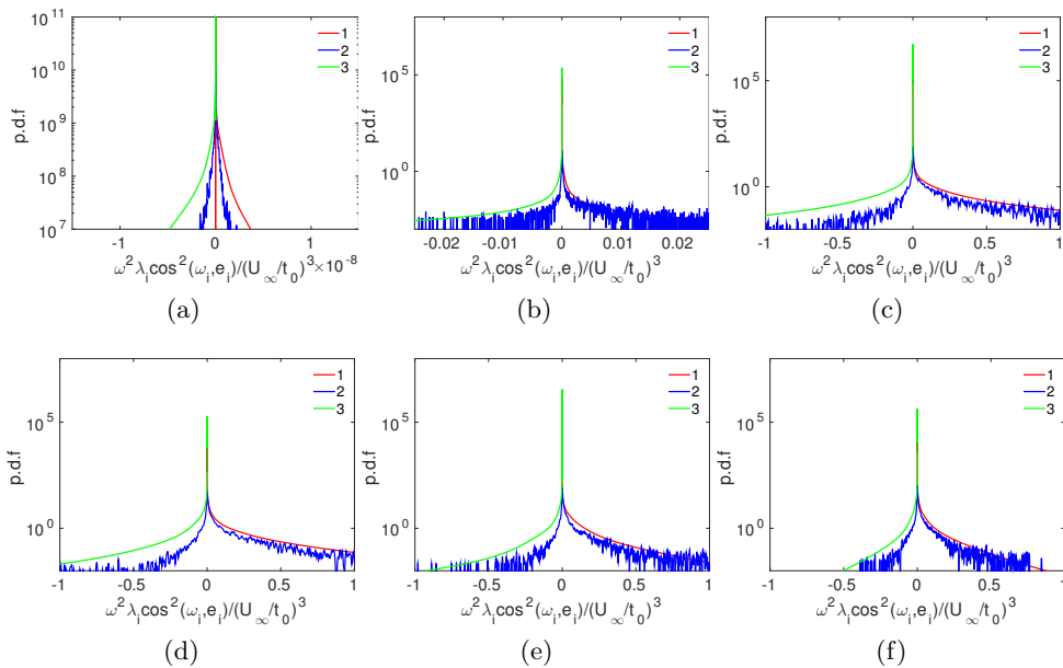
Figure 20: PDF of strain-rate eigenvalues contribution to enstrophy production at different locations along the grid-element centreline: (a) x/x^*=0.1 , (b) x/x^*=0.25 , (c) x/x^*=0.35 , (d) x/x^*=0.5 , (e) x/x^*=0.75 , (f) x/x^*=0.95 .
