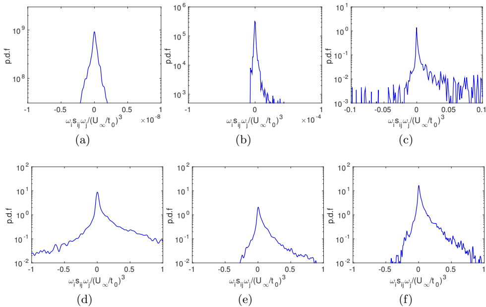
Figure 14: PDF of enstrophy production at different locations along the grid-element centreline: (a) x/x^*=0.1 , (b) x/x^*=0.25 , (c) x/x^*=0.35 , (d) x/x^*=0.5 , (e) x/x^*=0.75 , (f) x/x^*=0.95 .
