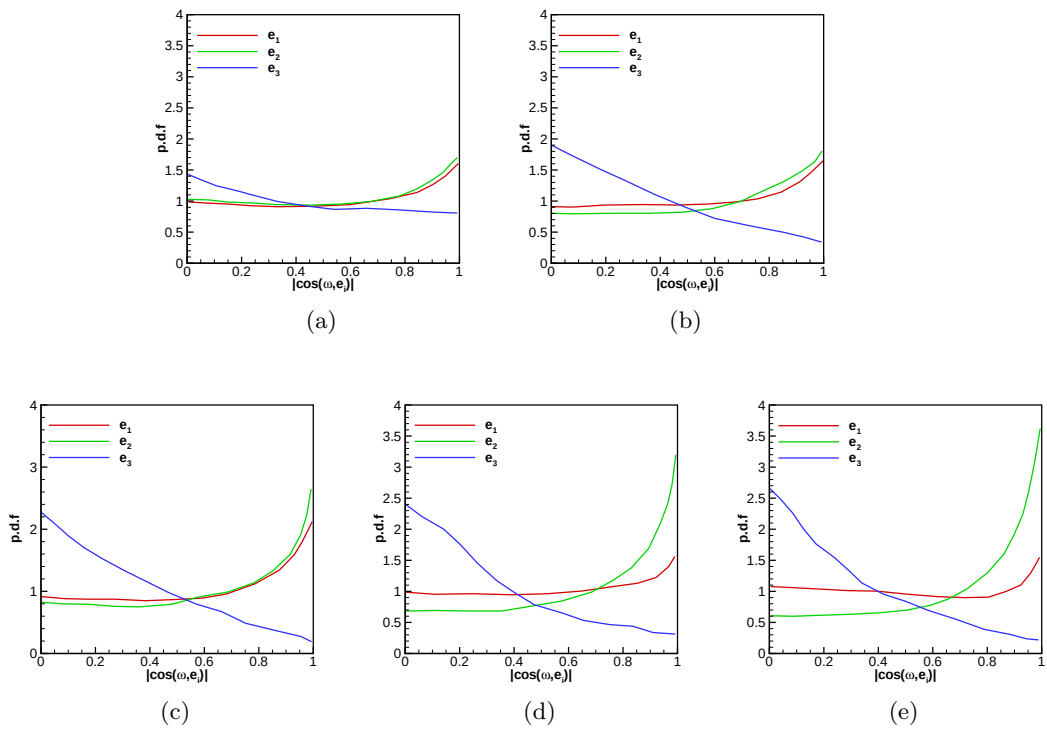
Figure 22: PDF of absolute value of the cosine of the angle between the vorticity vector and the eigenvectors of the strain-rate tensor at different locations along the grid-element centreline: (a) x/x^*=0.25 , (b) x/x^*=0.35 , (c) x/x^*=0.5 , (d) x/x^*=0.75 , (e) x/x^*=0.95 .
