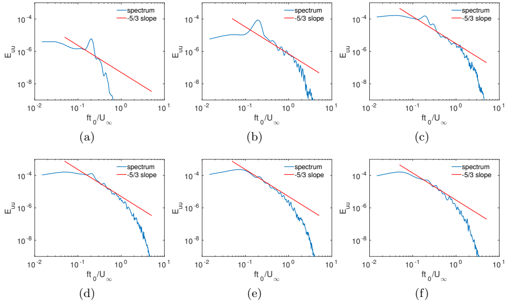
Figure 13: Energy spectra at different locations along the grid-element centreline: (a) x/x^* = 0.1 , (b) x/x^* = 0.25 , (c) x/x^* = 0.35 , (d) x/x^* = 0.5 , (e) x/x^* = 0.75 , (f) x/x^* = 0.95 . The frequencies f have been normalised with the ratio of the free-stream velocity U_\infty and the thickness t_0 .
