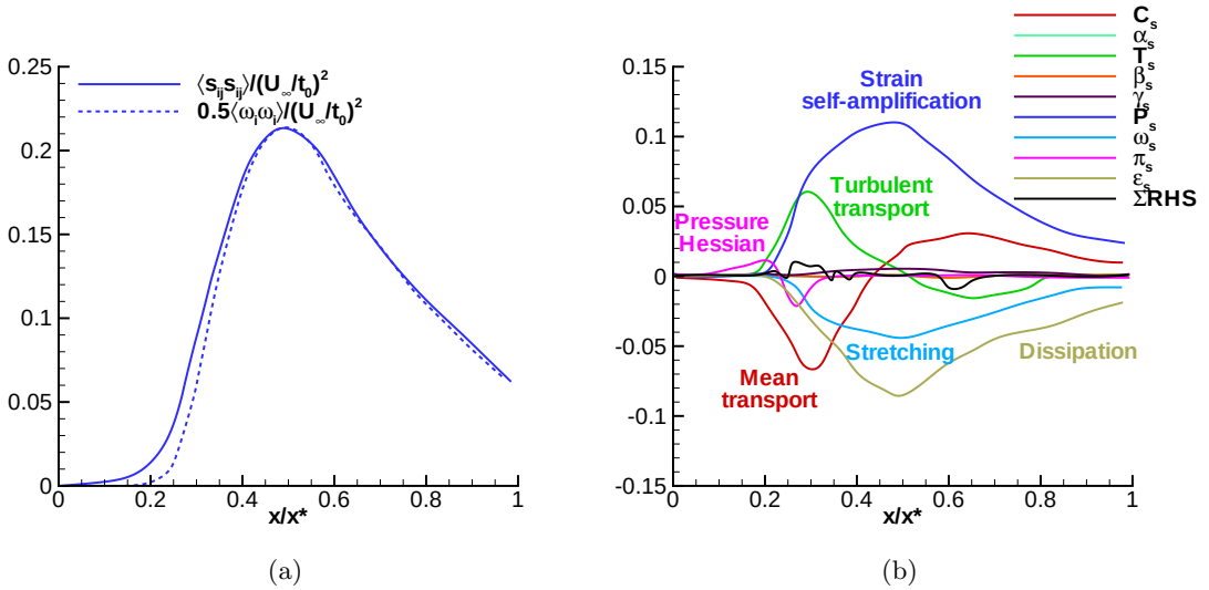
Figure 10: (a) Evolution of mean strain-product along the grid-element centreline (b). Budget of mean strain-product along the grid-element centreline (all terms are normalised by (U_\infty/t_0)^3 ).
