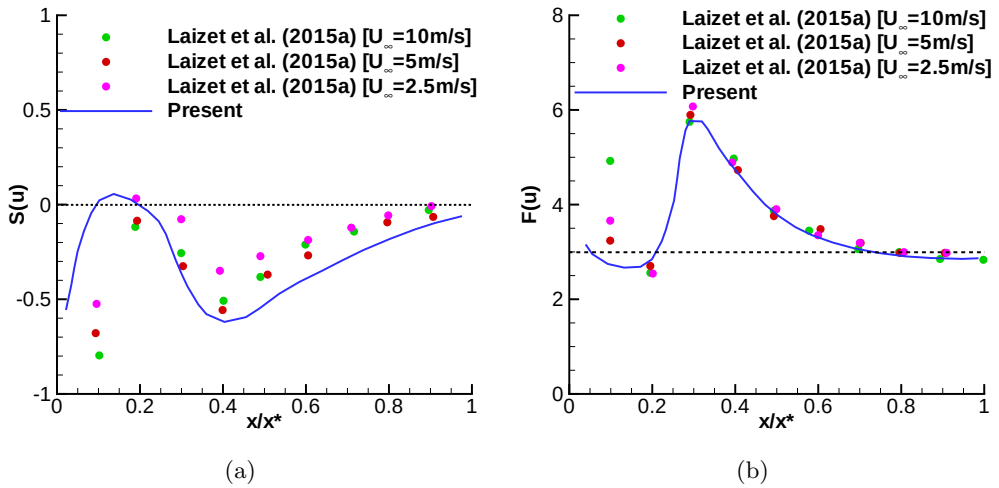
Figure 5: Comparison of (a) skewness and (b) flatness of streamwise fluctuating velocity along the grid-element centreline with experiments.
