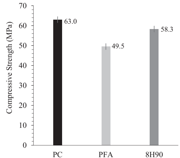
Fig. 10. Compressive strength at 28 days of PC mortar prisms with 25 % PFA and AAS subjected to 8 hour treatment in 5 M HCl at 90 °C. Error bars show 95 % confidence interval.
