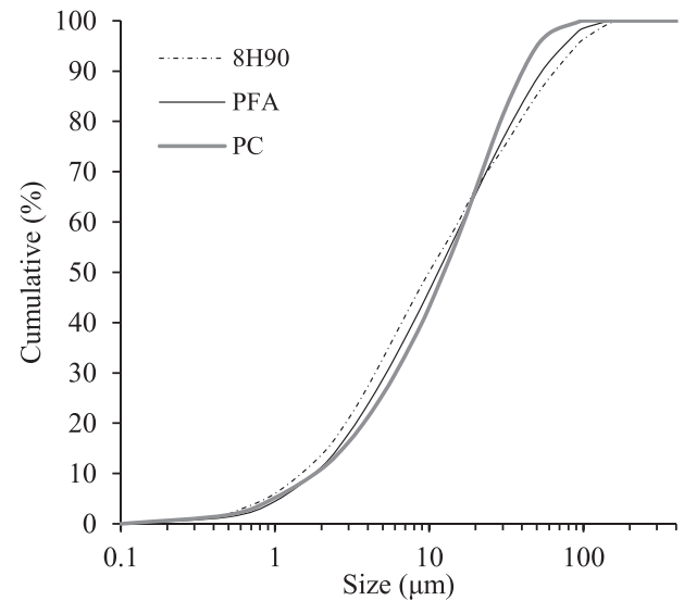
Fig. 9. Particle size distribution of PC, PFA and 8H90 AAS sample.
