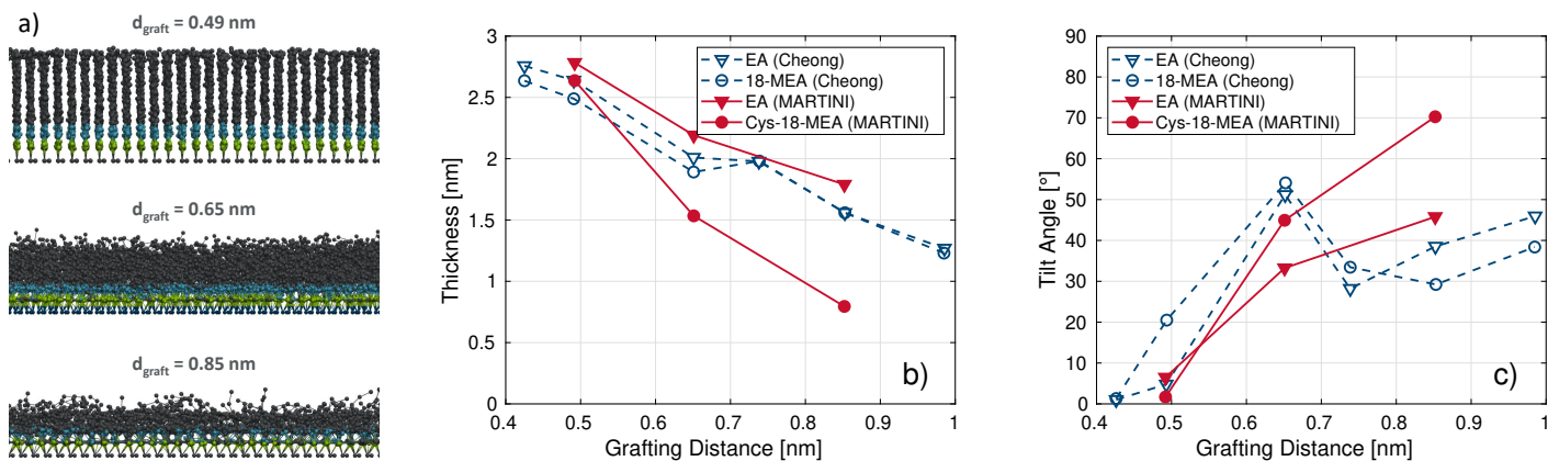
Fig. 2 Snapshots of Cys-18-MEA lipid monolayers at different grafting distances rendered using VMD 96 a). C_1 beads are shown in black, C_5 in blue, and P_5 in green. EA and Cys-18-MEA monolayer b) film thickness and c) tilt angles compared to AA-MD reference data for EA and 18-MEA from Cheong et al. 37 . Lines are guides for the eye. The thickness and tilt angles are measured from the centre of mass of the N_a bead to the terminal C_1 bead for EA and the P_5 bead to the terminal C_1/C_2 bead for Cys-18-MEA.
