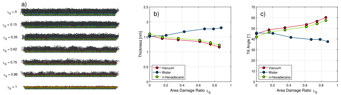
Fig. 3 Snapshots of monolayers in vacuum from \chi_S = 0 (top) to \chi_S = 1 (bottom) rendered using VMD. 96 a). C_1 beads are shown in black, C_5 in blue, and P_5 in green. Monolayer thickness b) and tilt angle c) at a nominal grafting distance of d_{\text{graft}} = 0.65 nm and various degrees of random damage in vacuum environment and with water and n -hexadecane. Lines are guides for the eye.
