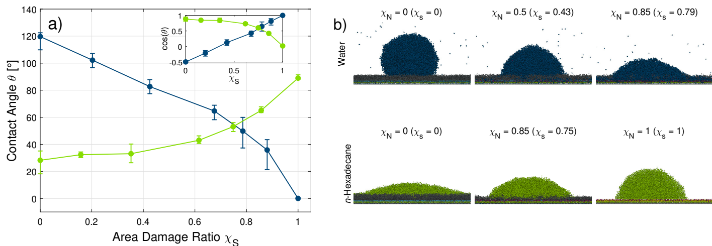
Fig. 6 Change in the water and n -hexadecane contact angles on model hair surfaces with an increasing degree of random damage a). Points show mean values from three different initial droplet positions and three different initial random damage seeds. Vertical bars show the minimum and maximum values observed across the temporal binning of the different position and seed trials. Solid lines are guides for the eye. Snapshots of water (blue) and n -hexadecane (green) droplets at low, medium, and high levels of damage rendered using VMD b). 96 Surface coverage ratios \chi_S are computed independently for monolayers with water and n -hexadecane. The inset shows the change in the cosine of the angle, rather than the angle.
