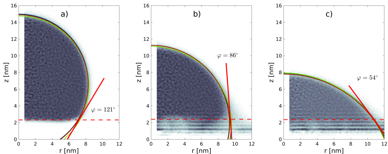
Fig. 5 Circular surface fits of a water droplets on the a) fully-functionalised, \chi_N = 0 , and partially damaged, b) \chi_N = 0.5 , c) \chi_N = 0.85 , monolayers from the CG-MD simulations. Four temporal bin fits for the droplet surface (solid circles) are shown. Averaged contact angles (solely from the shown four temporal bins) are indicated by bold red lines. The surface-normal position for the contact angle measurement is shown (dashed red line). Individual surface density fits in the radial direction are omitted for the sake of clarity. Note that the CG-MD simulation domain is larger than the radial section shown here.
