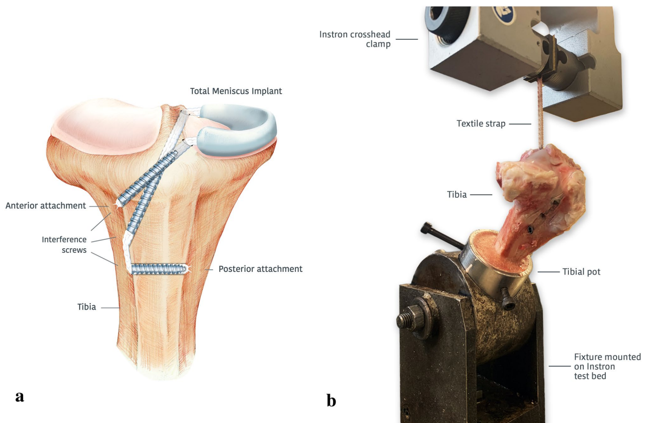
Fig. 1 Interference screw fixation of a total ovine medial meniscus replacement. a Anterior–posterior view with representation of the ovine medial meniscus implant fixation using interference screws within tibial bone tunnels. b Fixation testing setup for evaluating tex-
