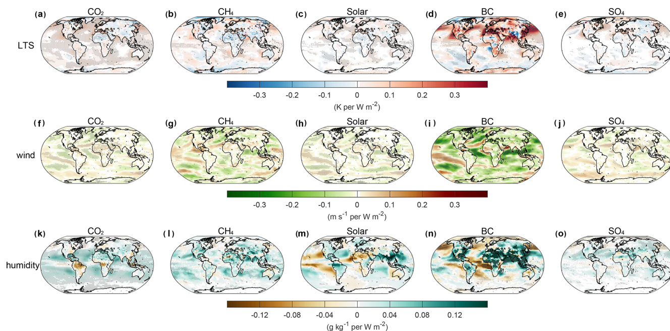
Figure 6. MMM changes for lower tropospheric stability (LTS, a–e ), surface wind velocity ( f–j ), and humidity gradient ( k–o ) per unit of global TOA forcing. For LTS, positive anomalies indicate a more stable atmosphere. The humidity gradient is defined as the specific humidity difference between the surface and 850 hPa. Grey dots indicate that the MMM changes are significant at a p value of 0.05.
