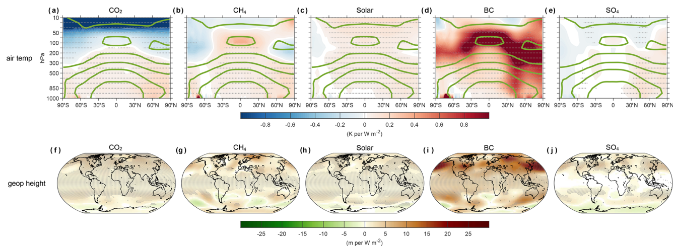
Figure 7. MMM changes for zonal atmospheric temperature ( a–e ) and geopotential height of 500 hPa ( f–j ) per unit of global TOA forcing. The thick green lines in the upper row are the climatology temperature in the control simulation. Grey dots indicate that the MMM changes are significant at a p value of 0.05.
