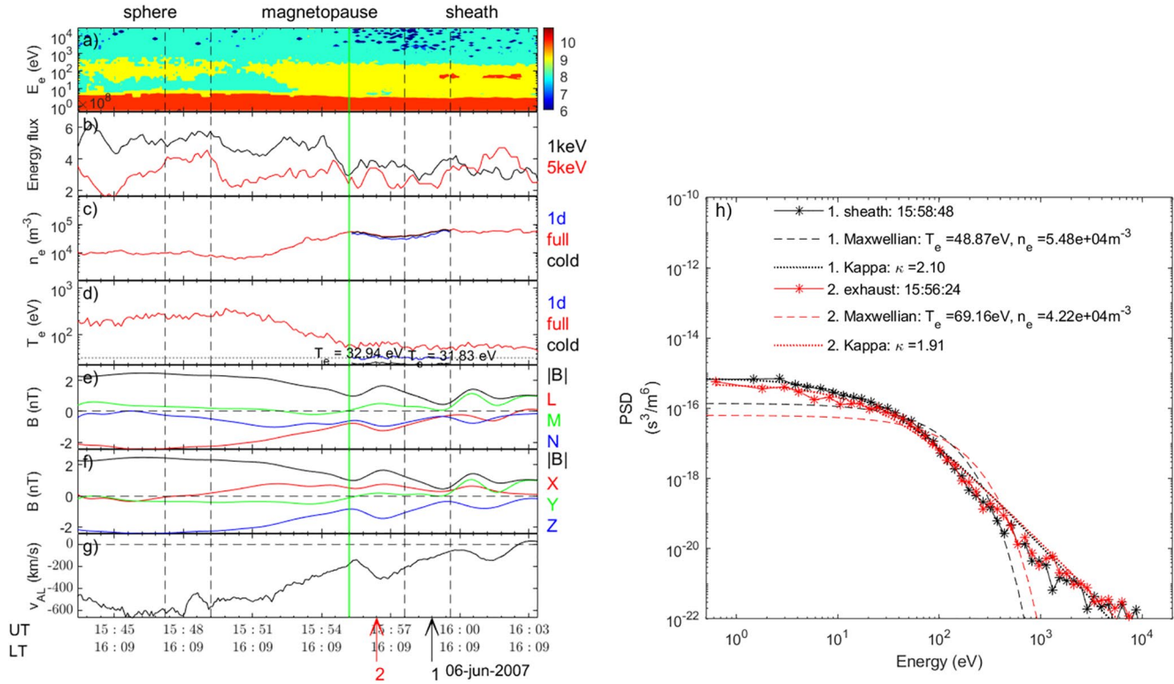
Figure 6. Exemplar magnetopause crossing without evidence of electron heating in category 3: Transitions without significant field rotation. The format of the panels is identical to Figure 4.
