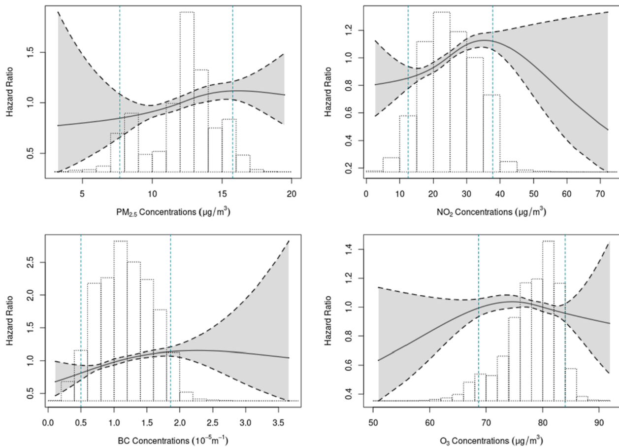
Fig. 2. Concentration-response curves for the association between long-term exposure to air pollution (PM 2.5 , NO 2 , BC, and O 3 ) and first-ever COPD hospitalization. Natural cubic splines with three degrees of freedom were fit for air pollutants to evaluate the linearity of the associations based on Model 3. Solid lines indicate hazard ratio values and dashed lines indicate their 95% confidence intervals. Green dashed lines indicate 5th and 95th percentiles of air pollutants' concentrations. (For interpretation of the references to colour in this figure legend, the reader is referred to the web version of this article.)
