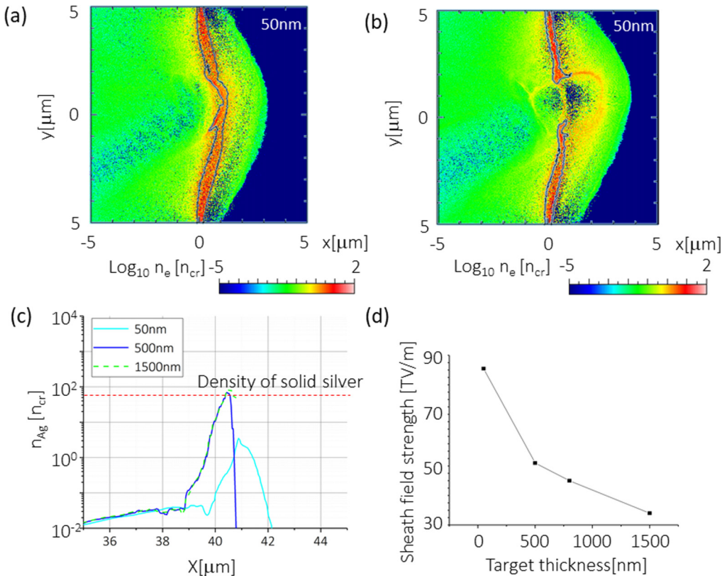
FIG. 9. Electron density profile in the PIC simulation for the 50 nm target at the time of (a) just before the main pulse irradiation and (b) 35 fs after the main pulse irradiation. The black lines shown in both panels indicate the position with density of \gamma n_{cr} . (c) Lineout of the initial silver density profile for the PIC simulation provided by the hydrodynamic simulation for each thickness of targets, i.e., light blue, blue, and dotted green show the cases of 50, 500, and 1500 nm targets, respectively. Initial position of the target front surface is located at X = 40 . The laser is irradiated from left-hand side to the target. (d) Sheath field strength from the PIC simulation against target thickness.
