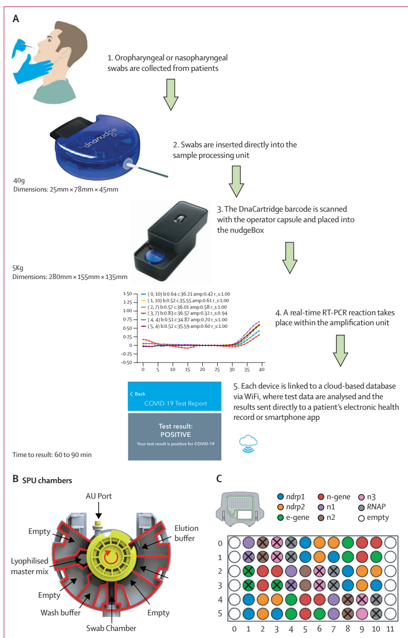
Figure 1: CovidNudge point of care diagnostic for SARS-CoV-2
