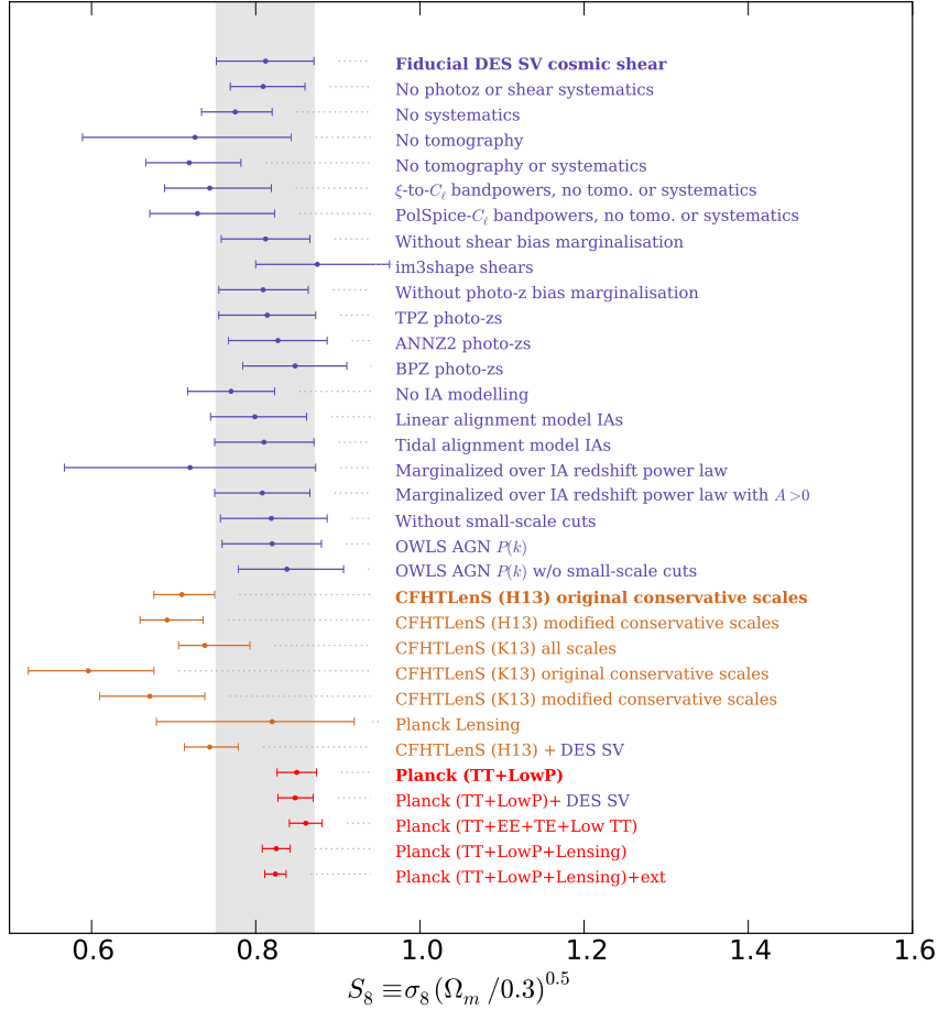
FIG. 3. Graphical illustration of the 68% confidence limits on S_8 \equiv \sigma_8(\Omega_m/0.3)^{0.5} values given in Table I, showing the robustness of our results (purple) and comparing with the CFHTLenS and Planck lensing results (orange) and Planck (red). The grey vertical band aligns with the fiducial constraints at the top of the plot. Note that Planck lensing in particular, and other non-DES lensing measurements optimally constrain a different quantity than shown above e.g. see the second and third columns of Table I.
