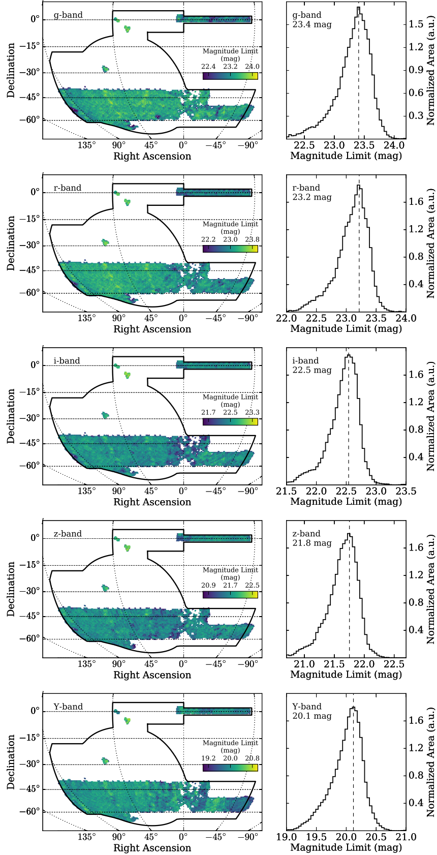
Figure C.1. Sky maps and normalized histograms of the 10\sigma limiting magnitude for galaxies fit with MAG_AUTO . The mode of the limiting magnitude distribution is shown in the right panel of each row. The derivation of the limiting magnitude is described in more detail in Section 7.1.
