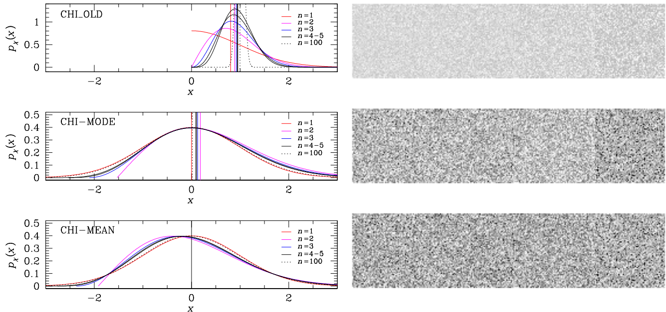
Figure B.1. (Left) Normalized distribution of the value x of a detection image pixel for the original \chi (OLD_CHI, top), CHI-MODE (middle) and CHI-MEAN (bottom) estimators when the inputs to the co-add are normally and independently distributed. n is the number of input images. The means of the distributions are shown as vertical lines. (Right) Gamma-corrected close-up of a \chi (OLD_CHI, top), CHI-MODE (middle) and CHI-MEAN (bottom) detection image computed from a set of 8 input images with zero-mean Gaussian white noise. The number of inputs decreases by steps of 64 pixels from left (eight inputs) to right (one input). CHI-MEAN detection images are virtually seamless, even at the transition between one and two input images.
