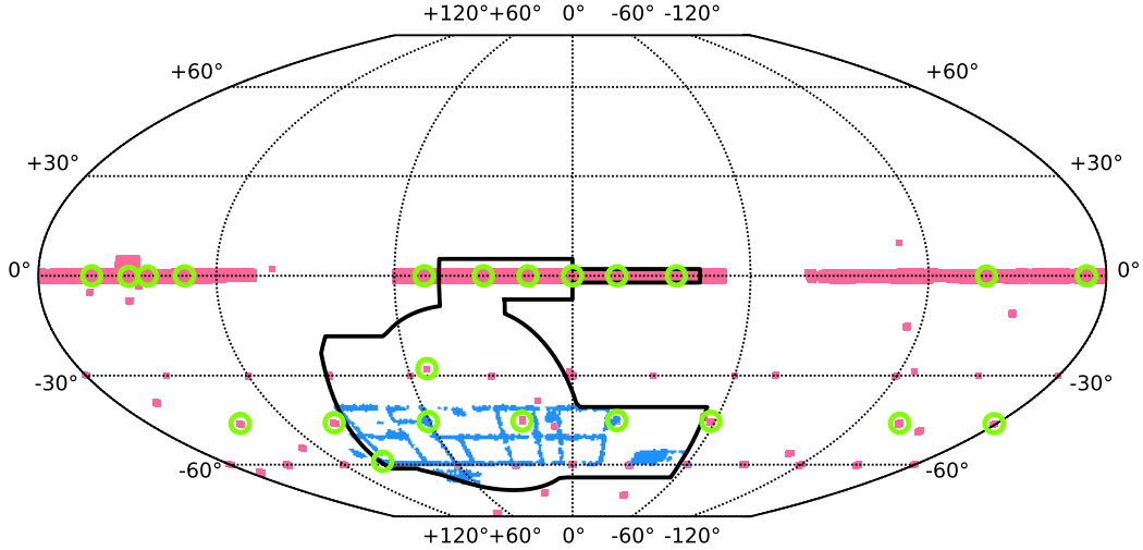
Figure A.1. Standard stars used for the photometric calibration of DES Y1. Nightly standard stars fields (Table A.1) are marked with green circles while other secondary standards from SDSS and Smith et al. (2017) are shown in pink. The grid work of tertiary standards is shown in blue.
