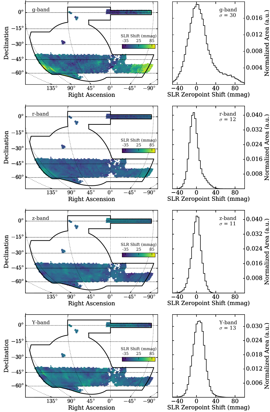
Figure A.8. Adjustment to the GCM photometric zeropoints derived from the SLR fit, after removing the contribution from interstellar extinction using the SFD maps and reddening from O’Donnell (1994). The width of these distributions represents adjustments to the calibration uniformity and differences between the interstellar extinction derived from the stellar locus and interstellar dust maps. The SLR adjustment is generally \sim 10 mmag (rms) over most of the area. A larger adjustment is made in the g band, which reflects the larger impact of reddening in the blue filters and a region of non-uniformity in the west of the footprint. There is no adjustment to the GCM i band because the SLR fit is tied to the dereddened magnitudes of stars in that band.
