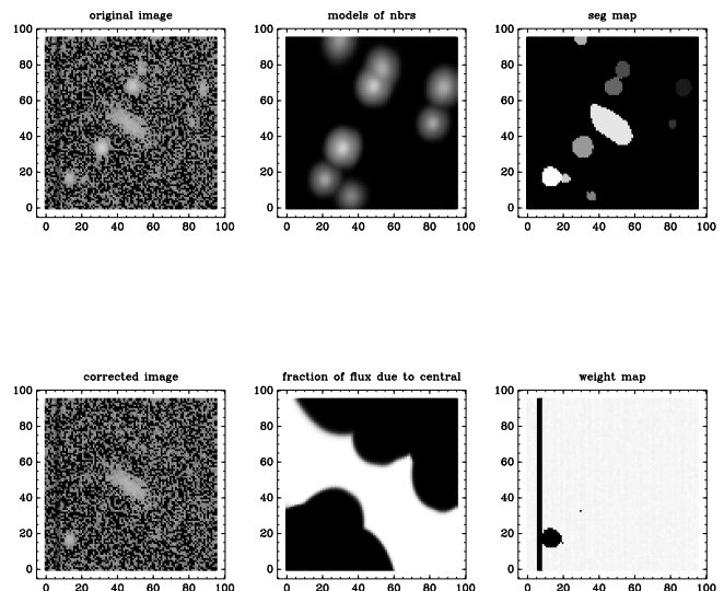
Figure 7. A group of objects fit using the MOF algorithm. In the top row we show: (left) the sky-subtracted image, (center) the models for neighboring sources, and (right) the SExtractor segmentation map. In the bottom row we show: (left) the sky-subtracted image after also subtracting the light from neighbors, (center) the fraction of light assigned to the central object (100% in white and 0% in black), and (right) the weight map. Note that a bad column and a flagged object are identified in the weight map. The masked object was not fit, and thus its light was not subtracted.
