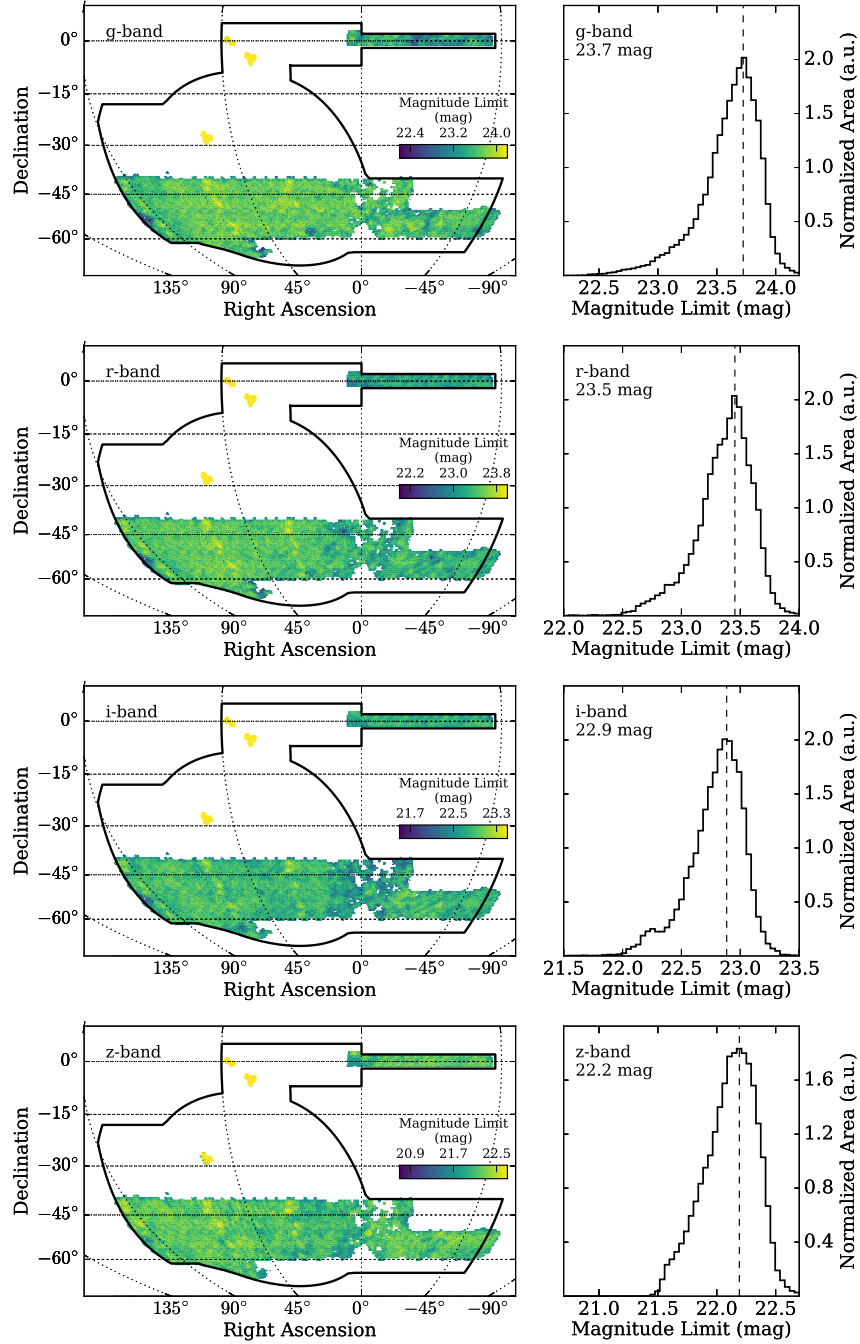
Figure C.2. Sky maps and normalized histograms of the 10\sigma limiting magnitude for galaxies fit with the MOF CM_MAG . The magnitude range for these figures is the same as the MAG_AUTO magnitude limits shown in Figure C.1. The mode of the limiting magnitude distribution is shown in the right panel of each row. Note that these magnitude limits include the deeper D10 coadds of the SN fields. The derivation of the limiting magnitude is described in more detail in Section 7.1.
