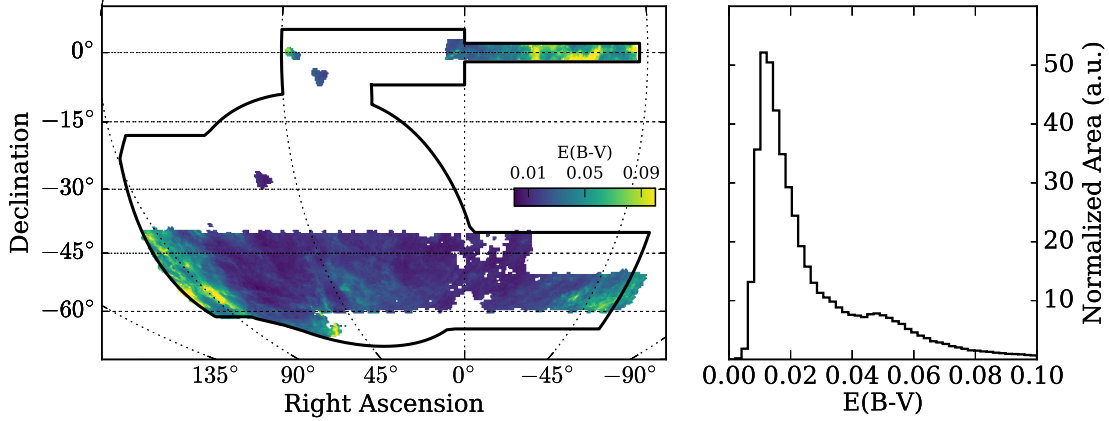
Figure A.5. Interstellar extinction, E(B - V) , over the Y1A1 GOLD footprint taken from Schlegel et al. (1998). The DES footprint was explicitly chosen to occupy a low-extinction region at high Galactic latitude.
