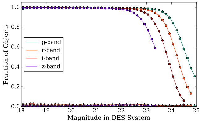
Figure 8. Completeness (solid circles) and contamination (dashed triangles) of the Y1A1 GOLD coadd object catalog determined by comparison to the CFHTLenS W4 field. Object matching was performed within a 1'' radius and CFHTLenS magnitudes were transformed to the DES system using the equations in Appendix A.4. Statistics were calculated for the subset of objects that were unmasked in both surveys and have been truncated at the 5\sigma limiting magnitude of CFHTLenS (Erben et al. 2013).
