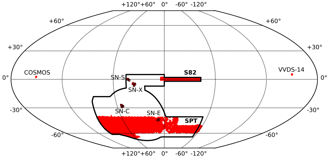
Figure 2. DES Y1A1 GOLD sky coverage in celestial coordinates (red) plotted in McBryde-Thomas flat polar quartic projection. Specific regions of Y1A1 GOLD footprint, including the SN and auxiliary fields, are explicitly labeled (see Section 2). The nominal DES five-year footprint is outlined in black.
