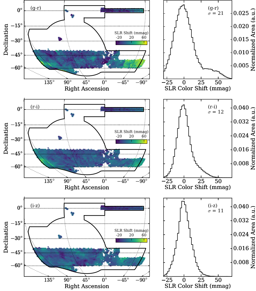
Figure A.9. Color uniformity of the SLR adjustment applied to the GCM zeropoints. The adjustment was largest for the (g-r) color in the eastern portion of the SPT region. The color non-uniformity in this region was one of the specific motivations for the SLR calibration adjustment. After the SLR adjustment was applied, the color of stars was found to be uniform at the 1–2% level across the footprint.
