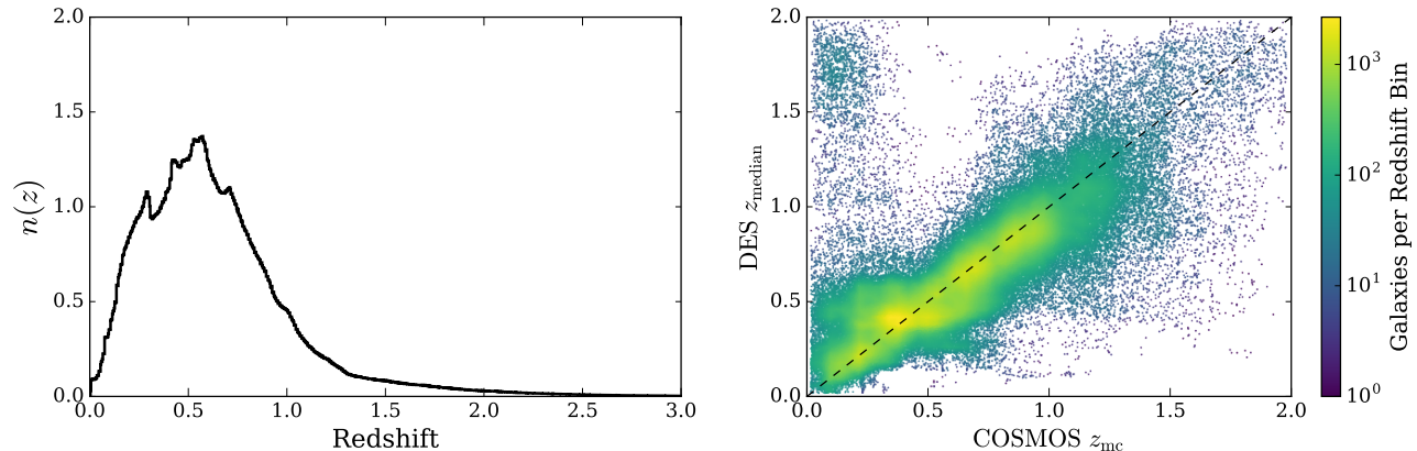
Figure 16. Performance of the BPZ photo- z estimates for the weak-lensing subsample of Y1A1 GOLD. (Left): The n(z) distribution generated from a random Monte Carlo sampling (i.e., Wittman 2009) of the BPZ P(z) distribution for each galaxy. (Right): Comparison between a random sampling of the 30-band COSMOS P(z) (Laigle et al. 2016) and the median of the DES BPZ P(z) for each galaxy in the overlapping sample. Points are colored by the local density of comparison galaxies in 0.04 \times 0.04 redshift bins.
