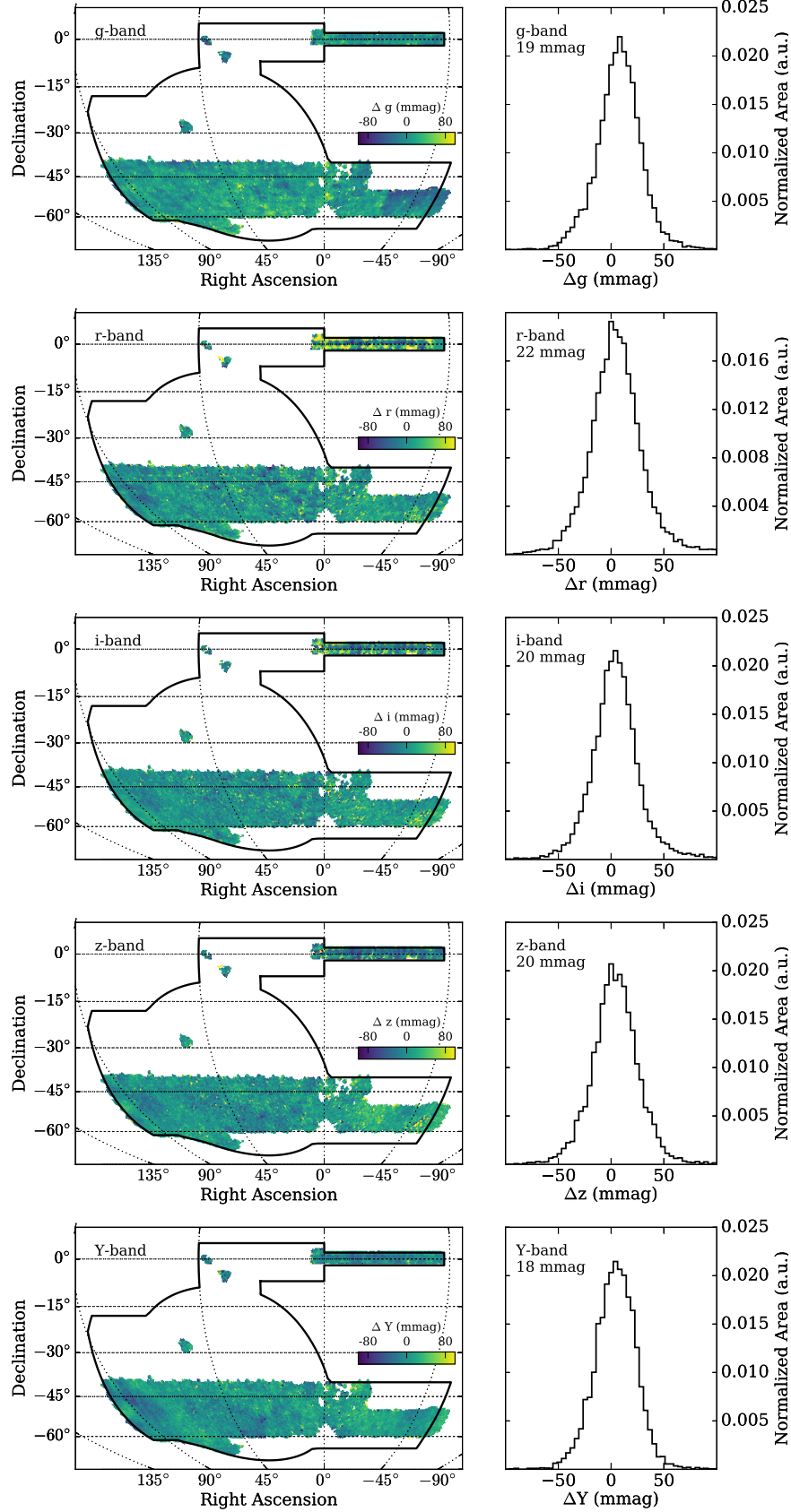
Figure A.7. Comparison of stellar magnitudes from the DES Y1A1 GCM and those estimated from APASS/2MASS transformed into the DES filter system (Equations A14-A18). The sky plots (left) show the median magnitude offset for stars binned into \sim 0.2 \text{ deg}^2 HEALPix pixels. The GCM calibrated magnitudes are consistent with the transformed values from APASS/2MASS with \sigma_{68} \sim 20 \text{ mmag} (calculated between the 16th and 84th percentiles). Note that the GCM g -band calibration disagrees with APASS/2MASS by \sim 4\% in the eastern portion of the SPT region ( \text{RA} < -20 ), motivating the SLR adjustment described in Section 4.3.
