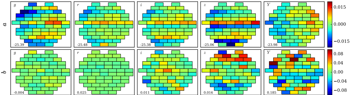
Figure A.2. Median fit values from DES Y1 for the a and b coefficients as a function of position on the DECam focal plane. The color scale represents the offset in the median fit value for each CCD with respect to the median for the focal plane as listed in the bottom left of each panel. The spatial variations in photometric zeropoints across the DECam focal plane are typically less than 0.02–0.03 mag for Y1A1.
