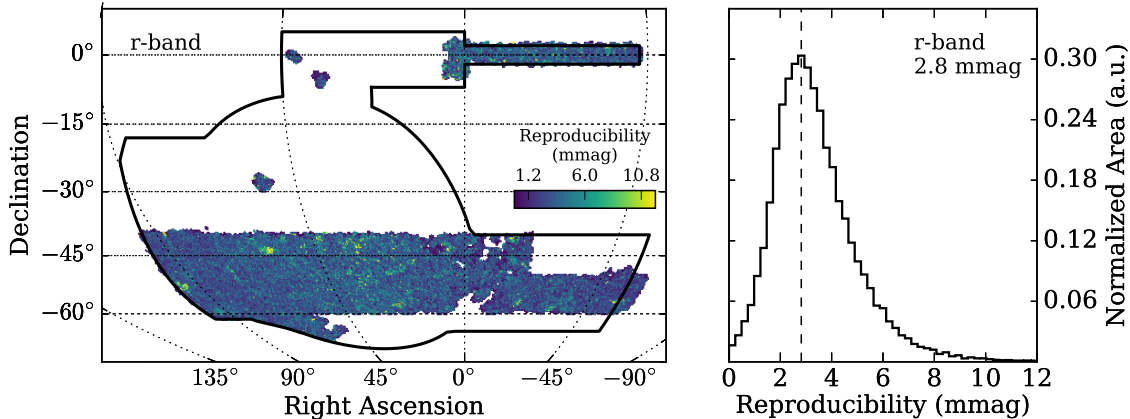
Figure 4. Internal reproducibility uncertainty for the Y1A1 r -band photometric zeropoints calculated by comparing the rms calibrated magnitudes of stars in overlapping CCDs. The mode of the rms internal calibration uncertainty is 2.8 mmag. Similar figures for other bands are shown in Appendix A.2.
