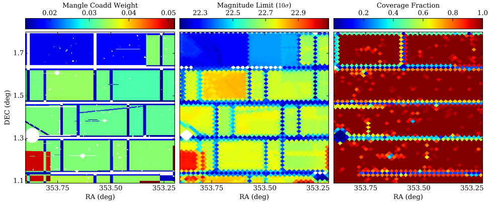
Figure 9. Coverage and depth maps for a single Y1A1 coadd tile. (Left) Vectorized mangle weight map for an r -band coadd tile. Satellite trails, star masks, and chip gaps are stored at full resolution. (Center) Pixelized 10\sigma limiting magnitude map for galaxies using HEALPix at nside = 4096. (Right) Pixelized map of the coverage fraction at HEALPix nside = 4096. This tile is located on the border of the Y1A1 footprint and has been chosen for illustrative purposes due to its variable depth and incomplete coverage.
