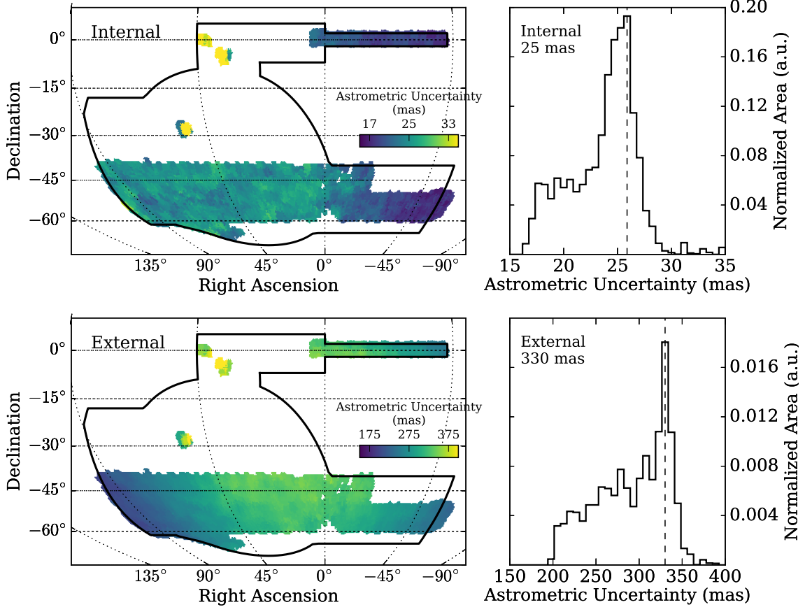
Figure 6. (Top): Relative internal astrometric error in milliarcseconds derived by comparing the positions of stars in the individual DES exposures that go into the Y1A1 coadds. (Bottom): Relative external astrometric error derived by comparing the position of stars in DES and 2MASS (without correcting for proper motion). The color scales represent the astrometric uncertainty in milliarcseconds, while the legends of the right panels report the modes of the distributions. The SN exposure times are significantly longer than the wide-area survey exposure times leading to a fainter saturation threshold. This reduces the number of non-saturated bright stars and increases the astrometric uncertainty estimated by this technique (a more accurate estimate of the astrometry in the SN fields can be found in Kessler et al. 2015).
