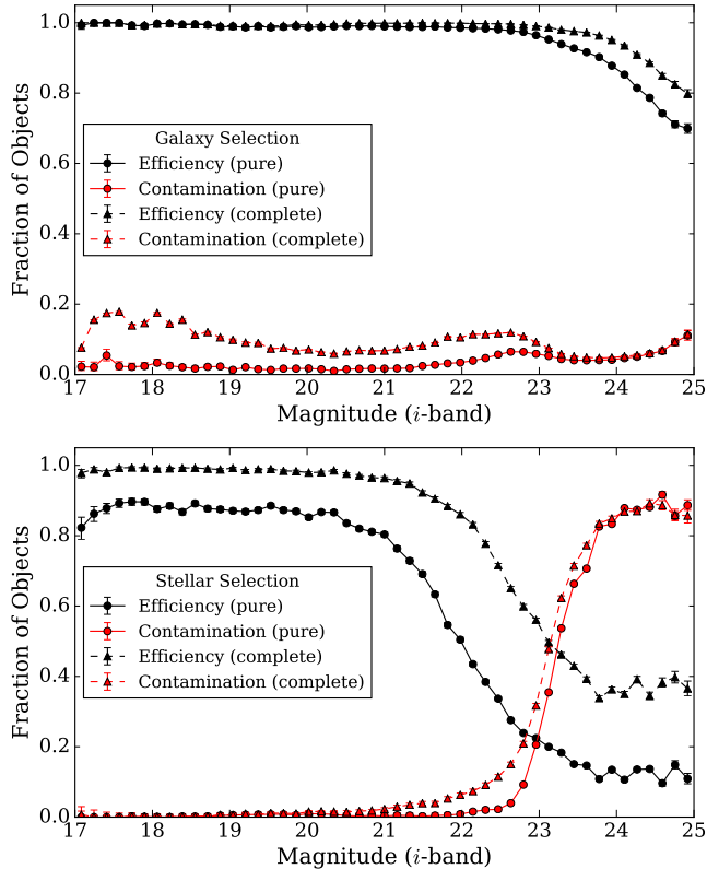
Figure 13. Performance of the MODEST_CLASS star-galaxy classifier based on a comparison to deeper imaging from CFHTLenS. (Top): The measured efficiency and contamination for high-purity (solid) and high-completeness (dashed) galaxy samples. (Bottom): The efficiency and contamination for high-purity (solid) and high-completeness (dashed) stellar samples (note that MODEST_CLASS is not optimized for stellar selection).
