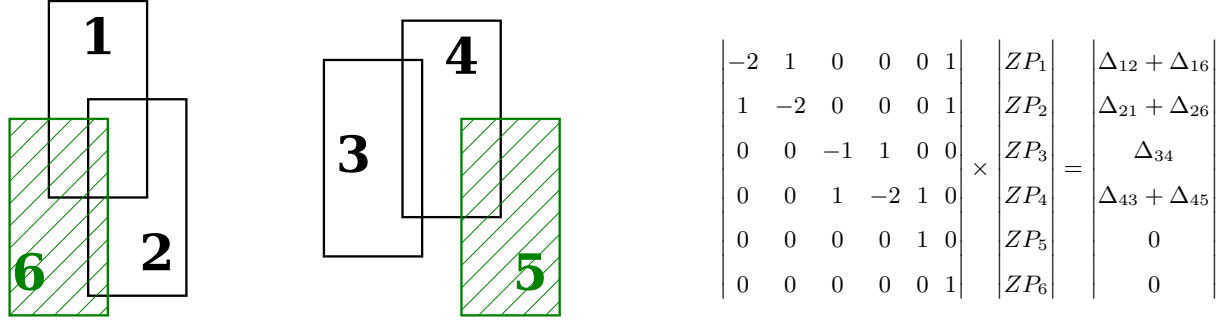
Figure A.4. A schematic of the GCM algorithm based on Fig. 1 of Glazebrook et al. (1994). Left: The stars in images 5 and 6 have been previously calibrated while the stars in the other images are uncalibrated. The algorithm minimizes the zeropoint offsets from all the overlapping images. Images that have a connected path via overlapping images to a reference image can be calibrated to that reference image. Right: The corresponding matrix equation for this set of images.
