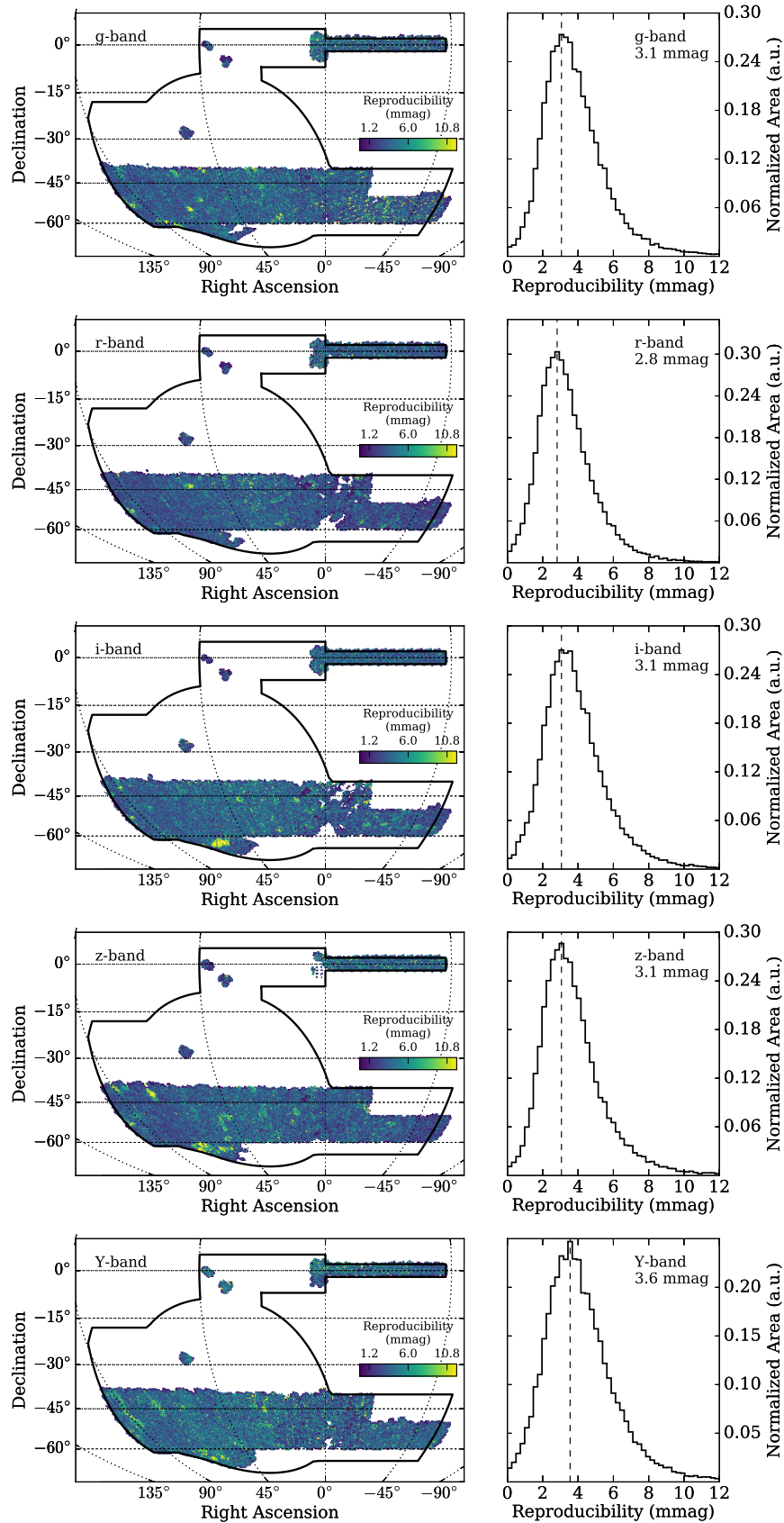
Figure A.6. Internal rms errors in the photometric zeropoint reproducibility per CCD for DES Y1A1. The zeropoint rms is calculated by comparing the calibrated magnitudes of stars in overlapping CCDs. Note that these data include observations taken in both clear and cloudy conditions. Typical internal reproducibility errors are \sim 3 mmag ( \sim 0.3\% ). The color scale in the left panels represents the rms internal calibration uncertainty in mmag.
