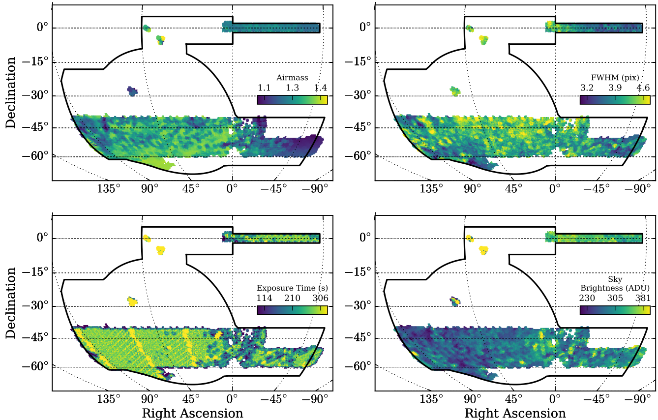
Figure 11. Survey characteristics of the Y1A1 GOLD data set estimated from the inverse variance weighted stack of single-epoch images in r -band at each position on the sky. Panels correspond to mean airmass (top left), PSF FWHM in pixels (top right), exposure time in seconds (bottom left), and sky brightness in ADU (bottom right).
