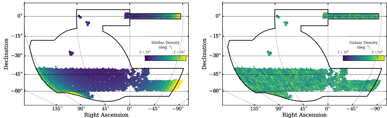
Figure 15. Density of objects with i < 22 passing the high-completeness star (left) and high-purity galaxy (right) MODEST_CLASS selections. The linear color scales represent the density of catalog objects and are the same for both panels. The density of objects has been corrected for the coverage fraction of each pixel (Section 7.1).
