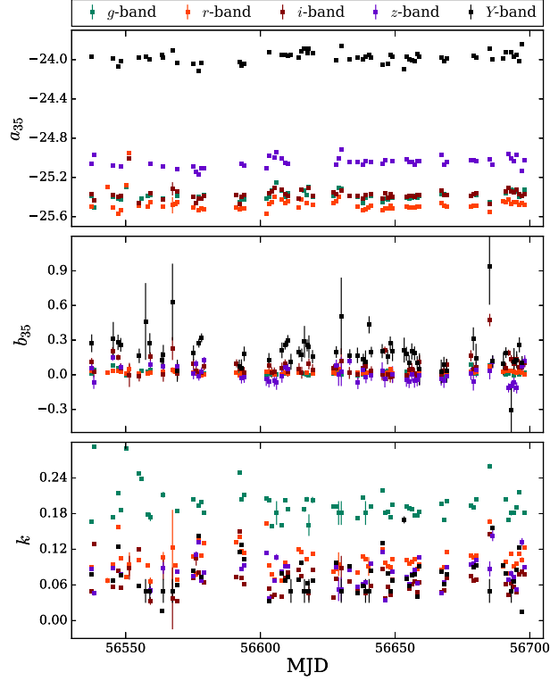
Figure A.3. Nightly fit values for the a coefficient of CCD35 (top), the b coefficient of CCD35 (middle), and the k coefficient of the DECcam focal plane (bottom) for nights in DES Y1. For the a and b coefficients, the trends in CCD35 are found to be representative of the trends in the other CCDs.
