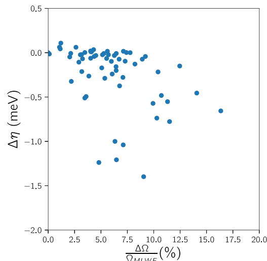
Fig. 7 \Delta\eta vs \Delta\Omega/\Omega^{\text{MLWF}} scatter plot (valence bands only). The dataset consists of the 81 insulators described in the main text (only 61 out of 81 visible in the axes range). \Delta\eta and \Delta\Omega/\Omega^{\text{MLWF}} represent the quantitative deviation between SCDM+MLWF and SCDM-only in terms of band structures and total spreads, respectively. Maximally-localised Wannier functions give comparable and often more accurate interpolated bands.
