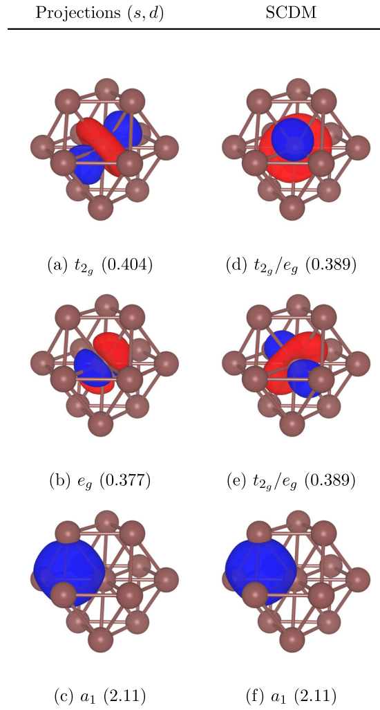
Fig. 2 MLWFs obtained by Wannierising the s - d complex in copper. First column: three representative MLWFs obtained from using atomic orbital projections to define the initial subspace (see main text for description). Panel (a) shows one of the three MLWFs with t_{2g} character; panel (b) shows one of the two MLWFs with e_g character; panel (c) shows one of the two broad s -like orbitals centred on a tetrahedral-interstitial site. Second column: three representative MLWFs obtained from using SCDM to define the initial subspace. Panels (d) and (e) show two of the five MLWFs with mixed t_{2g}/e_g character; panel (f) shows one of the two broad s -like orbitals centred on an tetrahedral-interstitial site. Below each function its individual spread in \text{Å}^2 is reported. Isosurfaces are plotted with an isovalue of \pm 0.45 \text{ Å}^{-3/2} .
