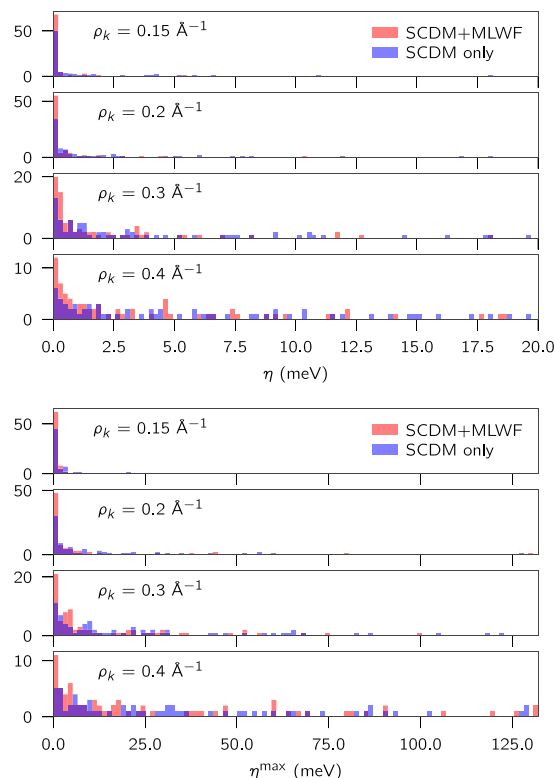
Fig. 3 Average and max band distance \eta using SCDM-only and SCDM+MLWF for the valence bands of 81 insulating materials.
