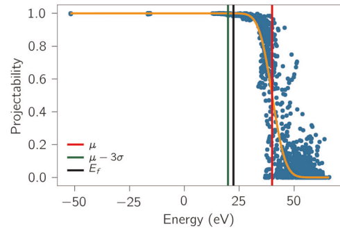
Fig. 8 Projectability of the state |nk\rangle as a function of the corresponding energy \epsilon_{nk} for tungsten. Each blue dot represents the projectability as defined in Eq. (22). The yellow line shows the fitted complementary error function. The vertical red line represents the value of \mu_{\text{fit}} while the vertical green line represents the optimal value of \mu , i.e., \mu_{\text{opt}} = \mu_{\text{fit}} - 3\sigma_{\text{fit}} . The value of the Fermi energy is also shown for reference (black line).
