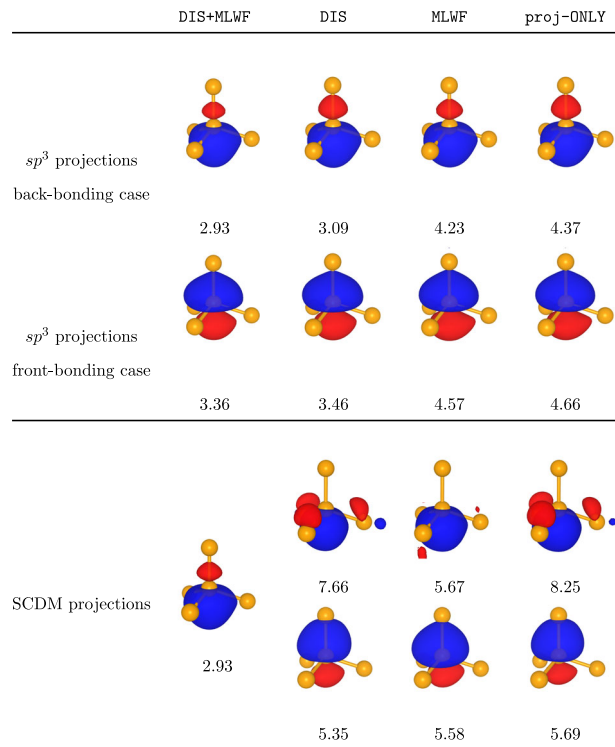
Fig. 1 Wannier functions obtained by Wannierising the four valence bands plus the four low-lying conduction bands in silicon.
