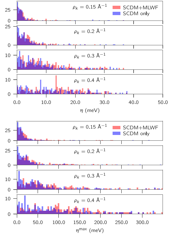
Fig. 11 Average and max band distance for the valence and few conduction bands of 200 materials. Top (bottom) panel: histogram of average (max) band distance \eta ( \eta^{\max} ) in meV using SCDM-only (blue) and SCDM+MLWF (red) obtained using four different k -point grids with spacing \rho_k . The MLWF procedure slightly worsens the accuracy of the interpolation when compared to SCDM-only Wannier functions. The histograms focus on the most relevant interval and few outliers are not shown, in particular at \rho_k = 0.2 \text{ \AA}^{-1} 98% (196/200) of the SCDM+MLWF bands and 99.5% (199/200) of the SCDM-only bands exhibit \eta < 50 meV, while 98% (195/200) of the SCDM+MLWF bands and 94% (188/200) of the SCDM-only bands exhibit \eta^{\max} < 350 meV.
