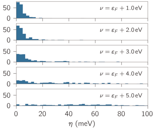
Fig. 10 Distribution of the band distance \eta for different values of the fictitious chemical potential \nu . The chemical potential is defined as \nu = \varepsilon_F + \Delta ( \Delta = 1, 2, 3, 4, 5 eV) and the smearing \tau in the Fermi–Dirac distribution is 0.1 eV. All calculations have been performed with a k -point spacing of \rho_k = 0.2 \text{ \AA}^{-1} .
