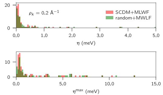
Fig. 5 Average and max band distance \eta using random+MLWF and SCDM+MLWF for the valence bands of 81 insulating materials. Top (bottom) panel: average (max) band distance \eta using random+MLWF (green) and SCDM+MLWF (red) obtained using \rho_k = 0.2 \text{ \AA}^{-1} . SCDM projections perform better than random projections when used in conjunction with the MLWF procedure. The histograms focus on the most relevant interval and few outliers are not shown, in particular the 96% (78/81) of the SCDM+MLWF bands and the 83% (67/81) of the random+MLWF bands exhibit an \eta < 5 \text{ meV} , while the 90% (73/81) of the SCDM+MLWF bands and the 74% (60/81) of the random+MLWF bands exhibit an \eta^{\max} < 15 \text{ meV} .
