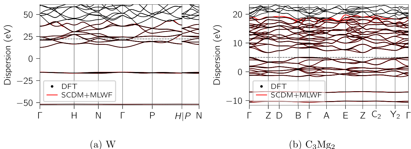
Fig. 12 Comparison between Wannier-interpolated valence bands plus few conduction bands and the full direct-DFT band structure. Wannier-interpolated bands are in solid red and full DFT bands are in solid black. Panel (a), \eta = 20 meV, \eta^{\max} = 415 meV, \mu = 19.85 eV and \sigma = 6.71 eV and C_3Mg_2 . Panel (b), \eta = 2 meV, \eta^{\max} = 11 meV, \mu = 0.86 eV and \sigma = 5.63 eV using the MLWF procedure on SCDM projections and \rho_k = 0.2 \text{ \AA}^{-1} . Note that, while we show all Wannier-interpolated bands, the band distance \eta considers only bands up to about 1 eV above the Fermi level (see text).
