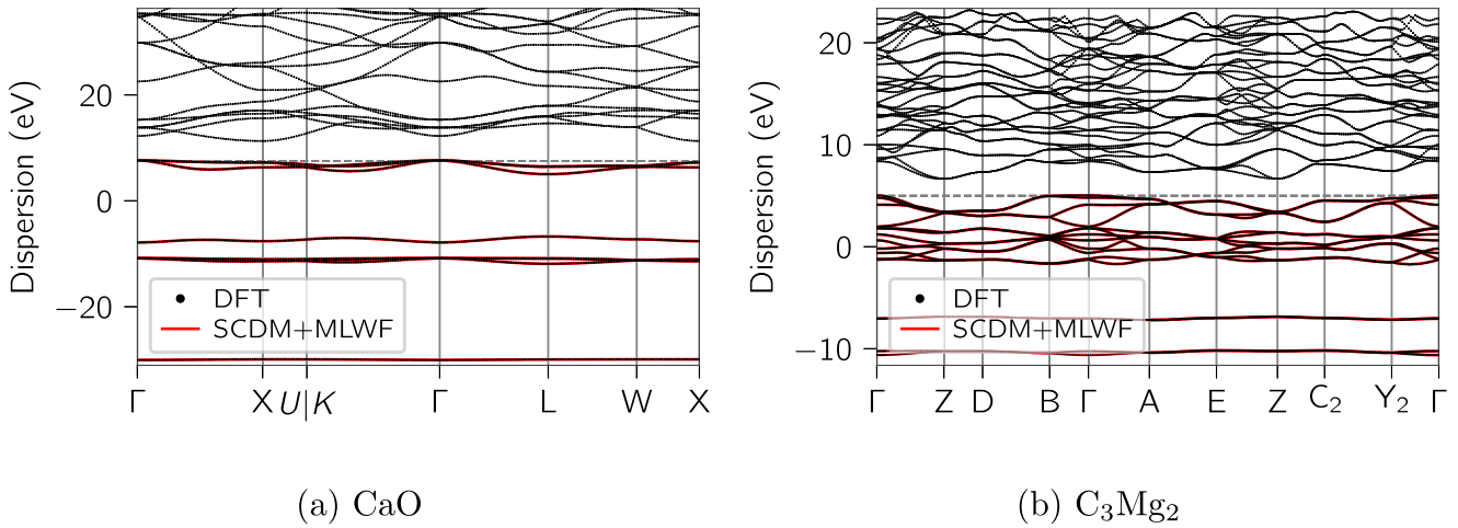
Fig. 4 Comparison between Wannier-interpolated valence bands and the full direct-DFT band structure. Wannier-interpolated (solid red) and full DFT band structure (black dots), using the MLWF procedure on SCDM projections and \rho_k = 0.2 \text{ \AA}^{-1} . The dashed line labels the valence band maximum (VBM). a Band structure of CaO ( \eta = 0.06 \text{ meV} , \eta^{\max} = 0.23 \text{ meV} , VBM = 7.52 eV). b Band structure of \text{C}_3\text{Mg}_2 ( \eta = 0.4 \text{ meV} , \eta^{\max} = 6.35 \text{ meV} , VBM = 5.0 eV).
