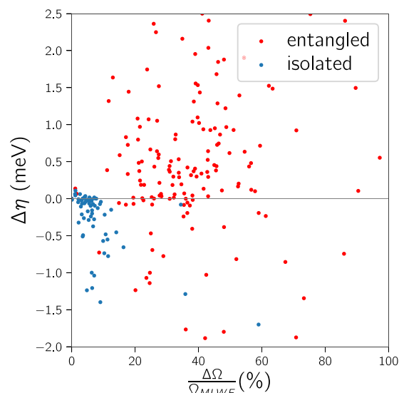
Fig. 14 \Delta\eta vs \Delta\Omega/\Omega^{\text{MLWF}} scatter plot (valence and few conduction bands). The dataset consists of all 200+81 materials, with entangled bands (red dots, 148 out of 200 visible in the axes range) and with isolated bands (blue dots, 64 out of 81 visible) showing \Delta\eta vs \Delta\Omega/\Omega^{\text{MLWF}} , that is the quantitative deviation between SCDM+MLWF and SCDM-only in terms of band structures and total spreads, respectively. Maximally-localising Wannier functions give potentially more accurate interpolated bands for valence bands only, whereas for entangled bands the trend is reversed.
