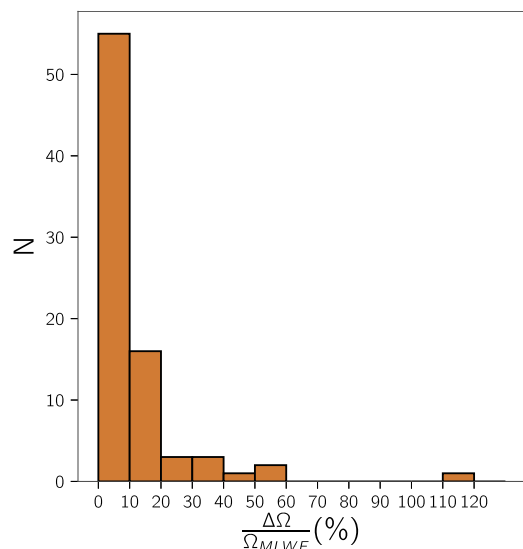
Fig. 6 Histogram of the relative variation of the total quadratic spread \Omega before and after the MLWF procedure. The data has been obtained considering the valence bands of our set of 81 insulators, with \rho_k = 0.2 \text{ \AA}^{-1} . The SCDM+MLWF procedure provides Wannier functions that are moderately more localised with respect to SCDM-only, with a relative variation within 10–20% for most materials.
