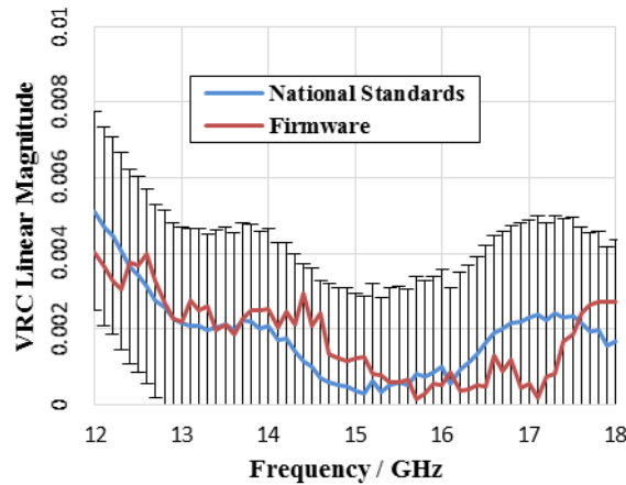
Figure 11. VRC linear magnitude for the near-matched load. Measurements made using: 3-D printed standards with a VNA’s firmware calibration and PIMMS using UK’s primary national standards.
