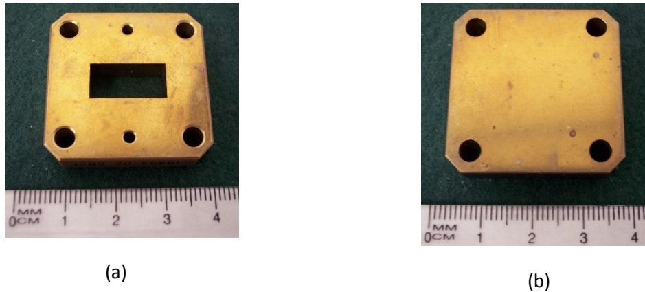
Figure 3. Photographs of the UK's primary national measurement standards: (a) \frac{1}{4} -wave line; and (b) short-circuit.
