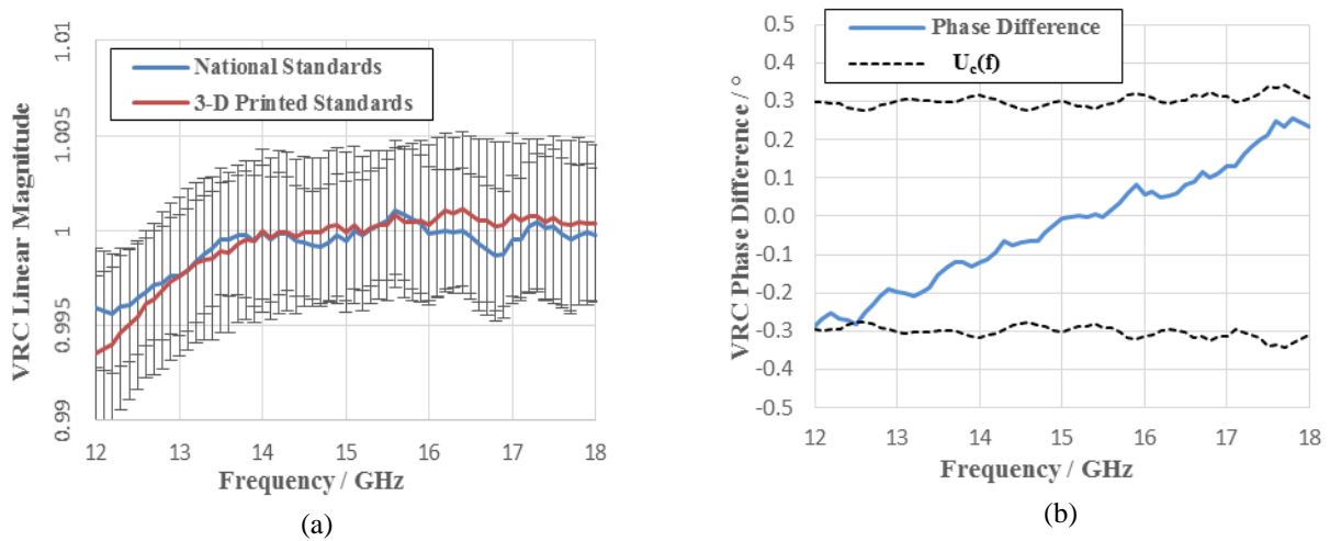
Figure 8. VRC for the offset short-circuit: (a) linear magnitude; and (b) phase difference between the two sets of measurements.
