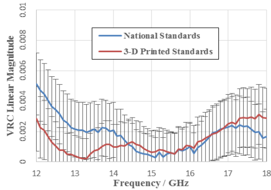
Figure 7. VRC linear magnitude for the near-matched load.
