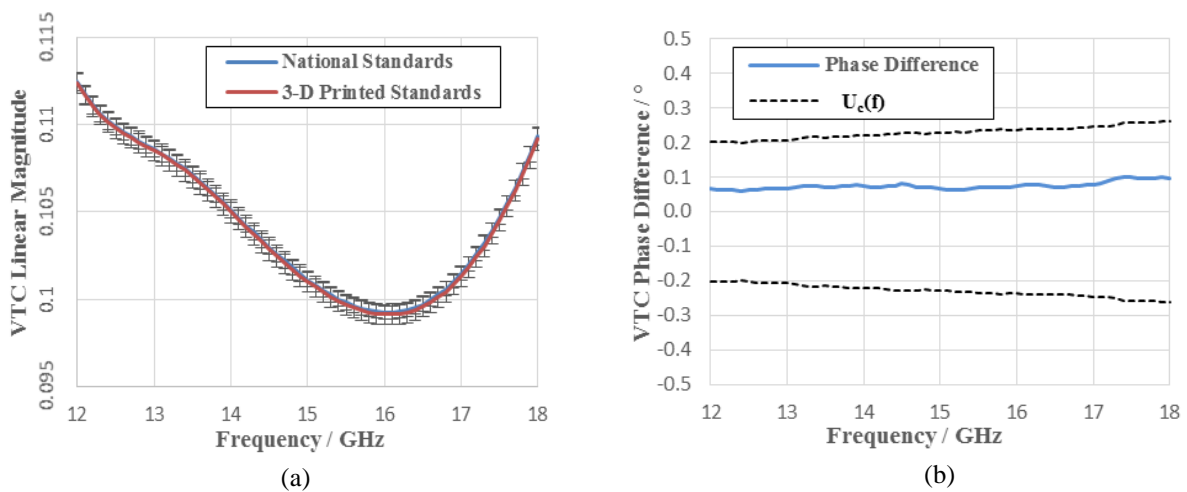
Figure 9. VTC for the 20 dB attenuator: (a) linear magnitude; and (b) phase difference between the two sets of measurements.
