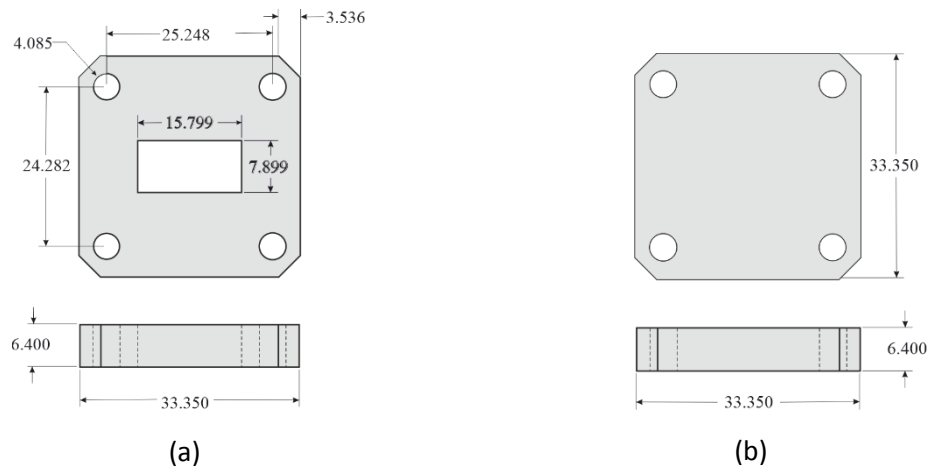
Figure 1. Engineering drawings showing the dimensions of the two Ku-band waveguide calibration standards: (a) \frac{1}{4} -wave line; and (b) short-circuit. All dimensions are in millimetres.
