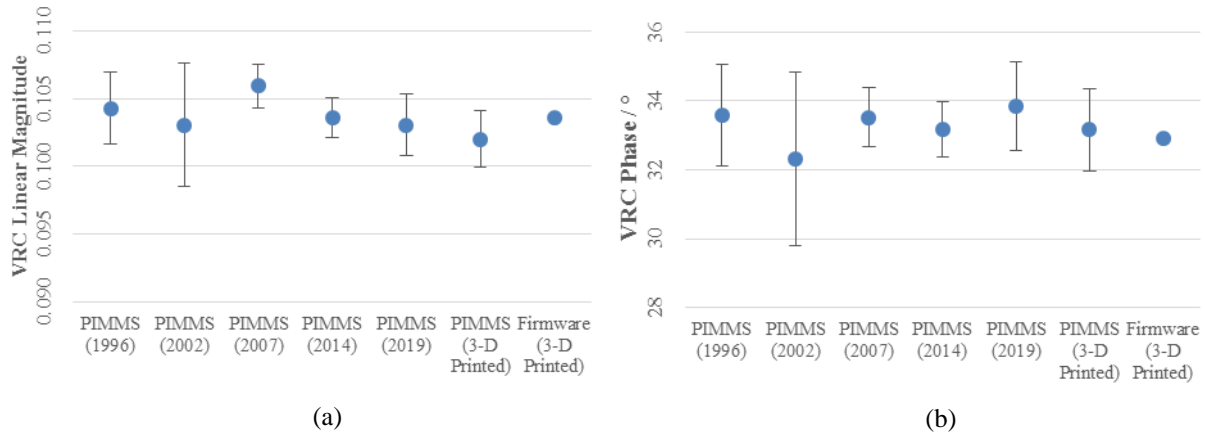
Figure 13. Historical VRC measurement data for the mismatched load verification device at 15 GHz: (a) linear magnitude; and (b) phase.
