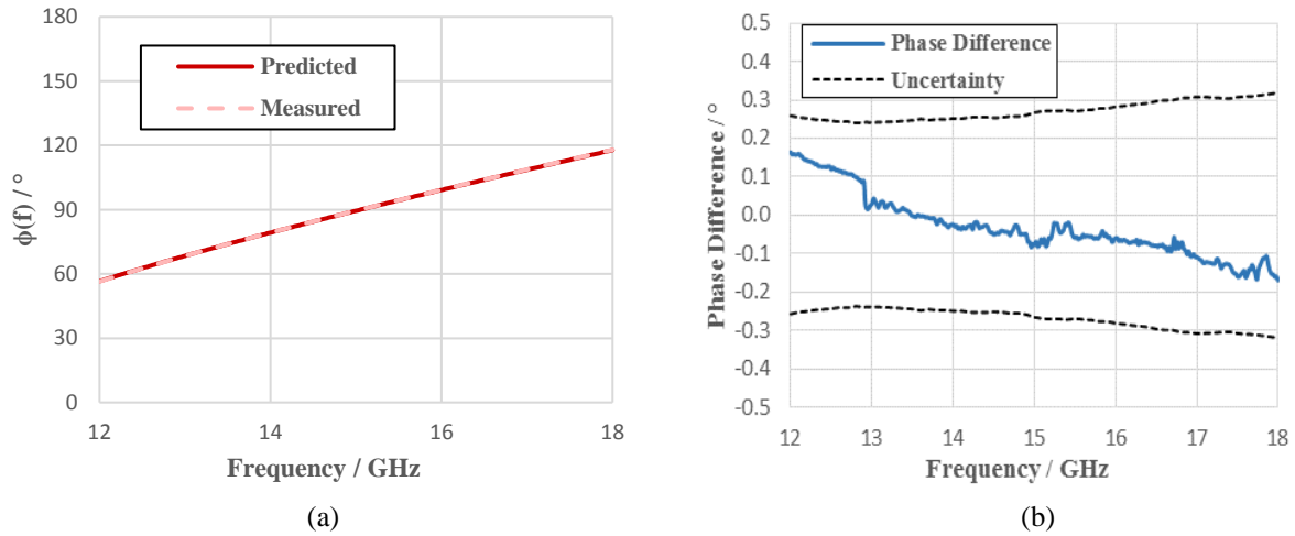
Figure 4. (a) Predicted and measured transmission phase for the 3-D printed line: (b) difference between predicted and measured transmission phase.
