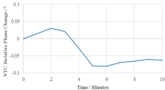
Figure 5. Change in VTC phase, measured at 15 GHz, relative to the VTC phase measured immediately after connecting the 3-D printed waveguide to the VNA.
