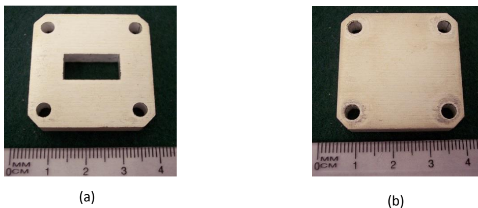
Figure 2. Photographs of the 3-D printed standards: (a) \frac{1}{4} -wave line; and (b) short-circuit.
