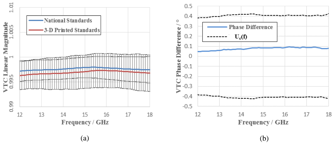
Figure 10. VTC for the 127 mm section of line: (a) linear magnitude; and (b) phase difference between the two sets of measurements.
