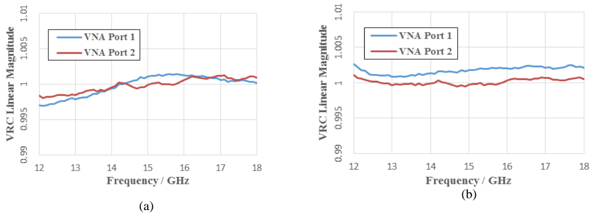
Figure 6. VRC linear magnitude measured using the two VNA test ports: (a) 3-D printed short-circuit; (b) conventionally machined short-circuit.
