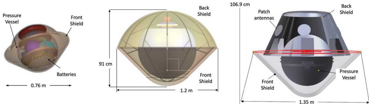
20 21 Figure 2. Probe designs from the 2010 Decadal study (left), 2017 NASA study (middle) and the 22 2018 ESA study (right). All employed a spherical pressurized descent vessel and \sim 45^\circ blunt-nose 23 front shield. However, the diameter and mass of the aeroshell have increased significantly since 24 the 2010 study.
