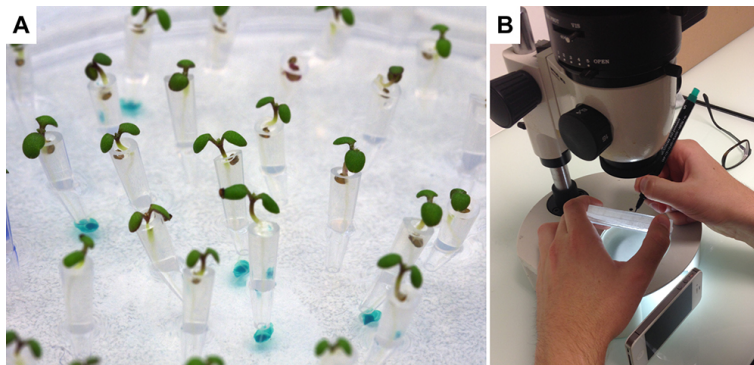
Figure 3. Arabidopsis seed farm. A. This photograph illustrates a “seed farm” that accommodates 5-day-old Arabidopsis seedlings germinated on agar-filled, cut pipette tips. The seed farm is created by placing Arabidopsis seeds on top of medium-filled pipette tips maintained in an agar plate. B. Prior to transfer onto the chip, seedlings with the proper root length are selected under a dissecting microscope (marked with blue dots on the bottom of the Petri dish in A).
