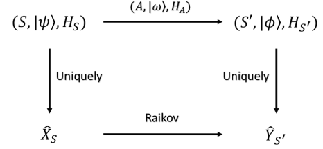
Figure 7: Raikov's theorem and coherent work processes. Given any quantum system S with Hamiltonian H_S in a state |\psi\rangle_X there is a unique classical random variable \hat{X}_S corresponding to the energy measurement on S . Conversely, given a random variable \hat{X}_S we may construct a (non-unique) tuple (S, |\psi\rangle_S, H_S) associated to this random variable.
