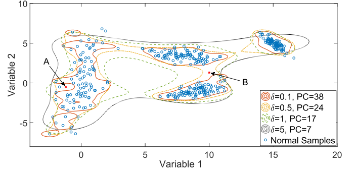
Fig. 4. Control limits of T^2 obtained by RBF kernels for training set 1.
