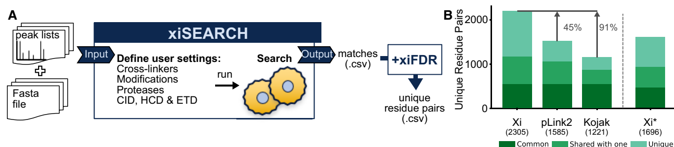
Figure 5. xiSEARCH.
