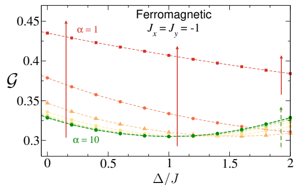
FIG. 2. (Color online.) Variation of genuine multipartite entanglement. Here, we consider a Heisenberg chain with N = 20 spins, and FM interactions ( J_x = J_y = -1 ) in the x - y plane. The plot shows the variation in \mathcal{G} with the parameter \Delta/J , where J = |J_x| = |J_y| , for ten different integer values of the exponent \alpha , ranging from \alpha = 1 (red-squares) to \alpha = 10 (green-circles). Here, the dashed lines are fits to the plotted data points. The regime \Delta = 0 corresponds to the XX model which also mimics the result obtained for Heisenberg chain at low \Delta . We note that the plots for higher \alpha values are very close together, which shows that the short-range character is reached fairly quickly. Moreover, the solid-red vertical arrows highlight specific parameter regimes where \mathcal{G} increases with decreasing \alpha (or increasing long-range interactions), whereas the dashed-green vertical arrows show regions where \mathcal{G} increases but now for increasing \alpha (or decreasing long-range interactions). Both the axes are dimensionless.
