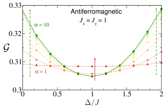
FIG. 3. (Color online.) Variation of genuine multipartite entanglement. Here, we consider a Heisenberg chain with N = 20 spins, and AFM interactions ( J_x = J_y = 1 ) in the x - y plane. The plot shows the variation in \mathcal{G} with the parameter \Delta/J (where, J = |J_x| = |J_y| ), for ten different integer values of the exponent \alpha , ranging from \alpha = 1 (red-squares) to \alpha = 10 (green-circles). Once more, the dashed lines are just fits to the plotted data points and both the axes here are dimensionless. The red and green vertical arrows here imply the same behavior as outlined in Fig. 2.
