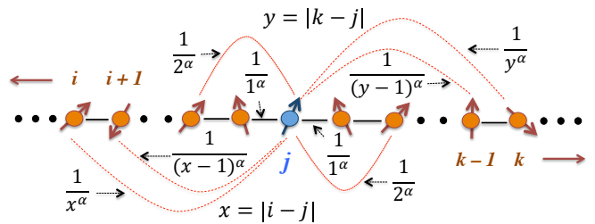
FIG. 1. Schematic of a quantum spin chain with interactions that follow a power-law decay, 1/r^\alpha . The black (bold) and red (dotted) lines show the short- and long-range coupling between the j^{\text{th}} and the other spins in the quantum system.
