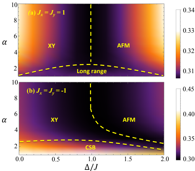
FIG. 4. (Color online.) Variation of genuine multipartite entanglement ( \mathcal{G} ) in the ground states of the long-range Heisenberg chain consisting of N = 20 spins in the \Delta/J - \alpha plane for (a) AFM and (b) FM interactions in the x - y plane. Here, J = |J_x| = |J_y| . We note here that the dashed yellow lines represent the extremal (minima) points of \mathcal{G} . However, they only serve as a visual aid to deconstruct the known quantum phases of the model (see Ref. [20]). Both the axes and the color bar in the figures are dimensionless.
