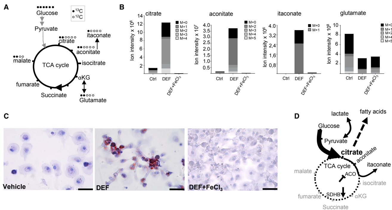
(A) Diagram of uniformly labeled [U]- 13 C-glucose catabolism, highlighting the TCA cycle metabolites and their expected glucose-derived 13 C atoms. (B) Stacked isotopologues measured by LC-MS shown for citrate, aconitate, itaconate, and glutamate in iron-deprived (DEF, 500 μM, 24 h) and rescued (DEF + FeCl 3 , 200 μM, 8 h) human macrophages with short exposure (8 h) to 200 μM ferric chloride (DEF + FeCl 3 ); n = 6 donors. (C) Vehicle, DEF-treated, or concomitant DEF and FeCl 3 -treated human macrophages stained for oil red O. The results are representative of n = 4 donors. (D) Summary of the TCA cycle changes due to iron deprivation in human macrophages. Citrate accumulation resulting from aconitase (ACO) inhibition and SDHB downregulation and the fate of citrate-derived metabolites are illustrated. Dashed circle represents inhibited TCA cycle activity. αKG, α-ketoglutarate. Scale bars, 40 μm. See also Figures S3 and S4.
