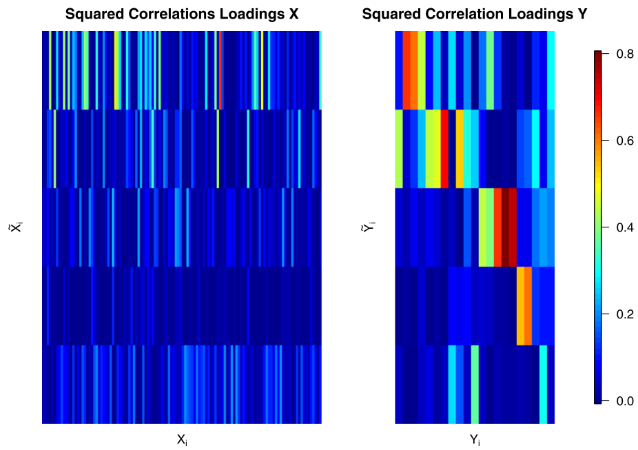
Fig. 4 Squared correlations loadings between the first 5 components of the canonical covariates \tilde{X}^{CCA} and \tilde{Y}^{CCA} and the corresponding observed variables X and Y for the Nutrimouse data
