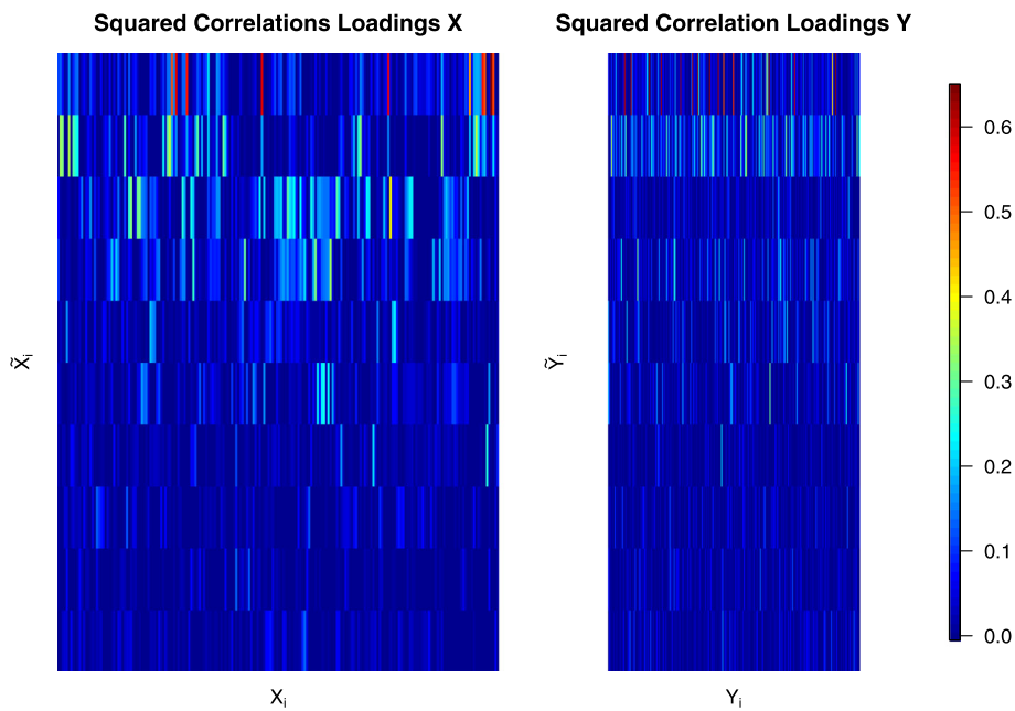
Fig. 8 Squared correlations loadings between the first 10 components of the canonical covariates \tilde{X}^{CCA} and \tilde{Y}^{CCA} and the corresponding observed variables X and Y for the TCGA LUSC data
