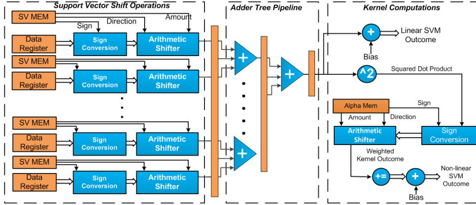
Fig. 5. Parallel Processing Module (PPM) Architecture: Handles the processing of the nearest power of two adapted SVM stages. The shift units and adder tree are used by all kernels while only non-linear kernels use the rest of the kernel module.
