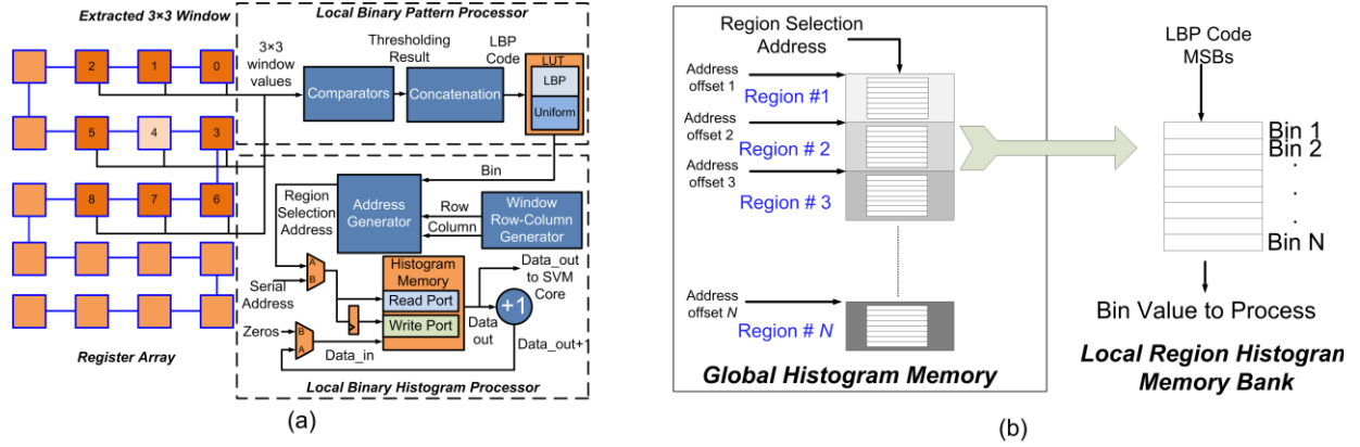
Fig. 7. (a) Local Binary Pattern Processor Architecture (b) Histogram Update Process
