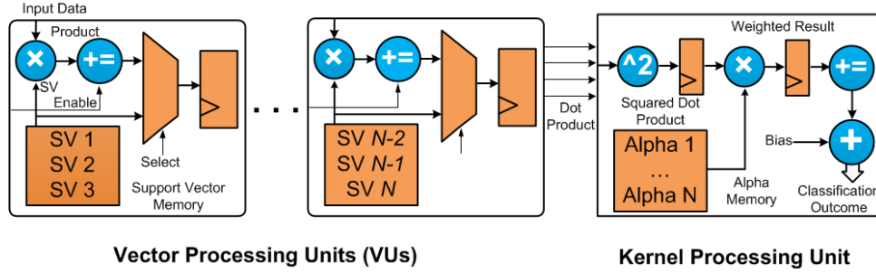
Fig. 6. Sequential Processing Module (SPM) Architecture: Consists of two processing units: The dot-product processing units handle the dot-product computation, and the kernel processing unit, which is shared amongst the dot-product units, handles the kernel-related operations.
