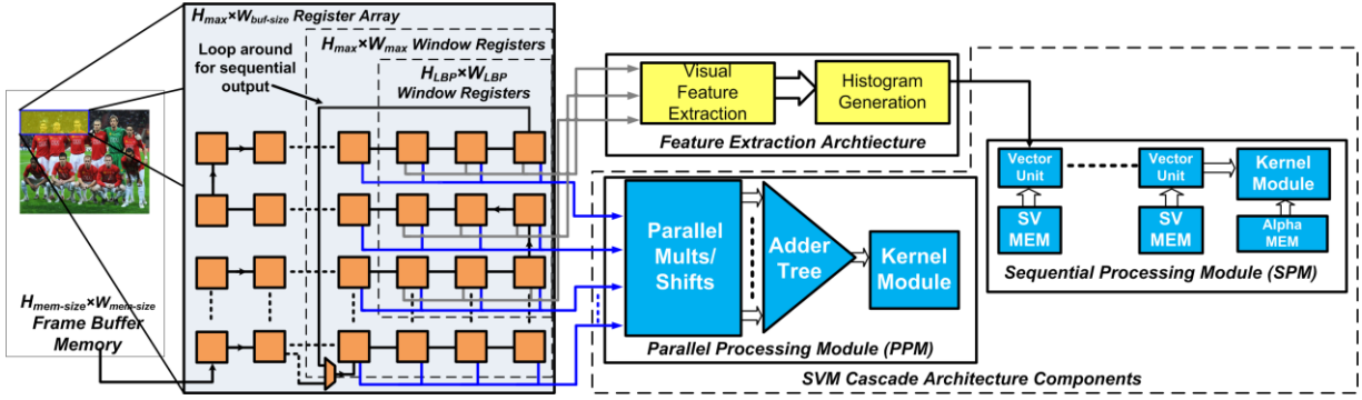
Fig. 4. SVM cascade system architecture comprised of the sequential processing module (SPM), the parallel processing module (PPM), the register array, frame buffer memory, and the visual feature processor.
