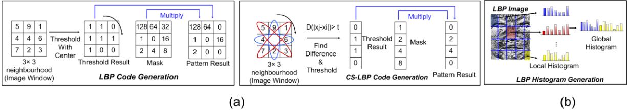
Fig. 2. Local Binary Patterns: (a) LBP Code generation using improved LBP and Center Symmetric LBP. (b) LBP histogram processing.
