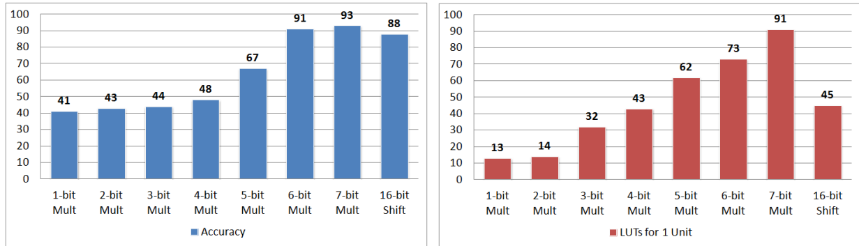
Fig. 12. Trade-off between accuracy and resources
