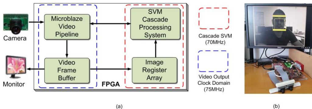
Fig. 8. (a) Block diagram of the FPGA system components. (b) Xilinx Spartan 6 FPGA industrial video processing board and setup for Face Detection Implementation
