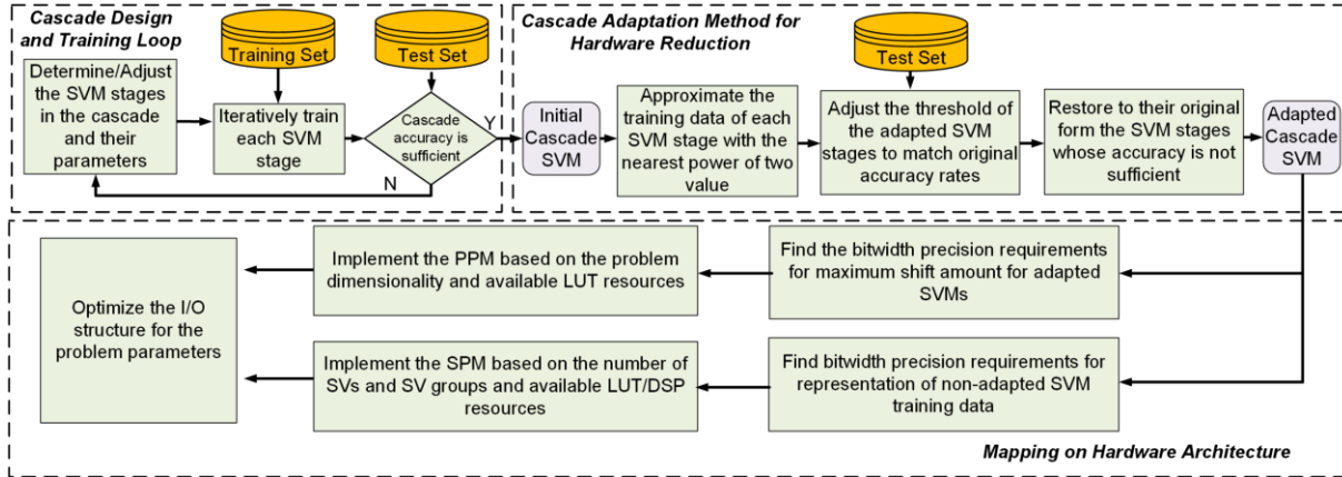
Fig. 3. Cascade Hardware Reduction Method: The initial cascade SVM obtained after training is altered to become more hardware friendly resulting in an adapted cascade SVM.
