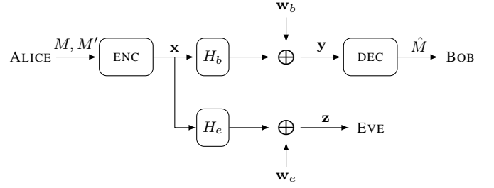
Fig. 1. The fading wiretap channel.
