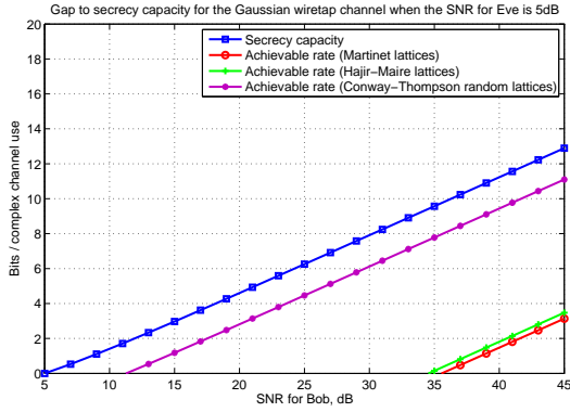
Fig. 3. Achievable rate on a single-antenna Gaussian wiretap channel, where the SNR for Eve is fixed at 5 dB.
