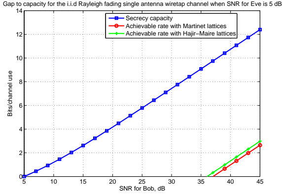
Fig. 2. Achievable rate for a single-antenna i.i.d. Rayleigh wiretap channel, where the SNR for Eve is fixed at 5 dB.
