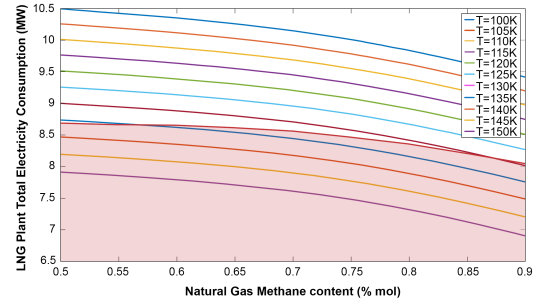
Fig. 6. Influence of the LNG composition in the available power for different product temperatures. The production rate in this simulation is 5000 tonnes per year.
