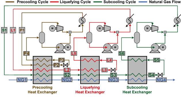
Fig. 2. Liquefied Natural Gas process using the Linde process
