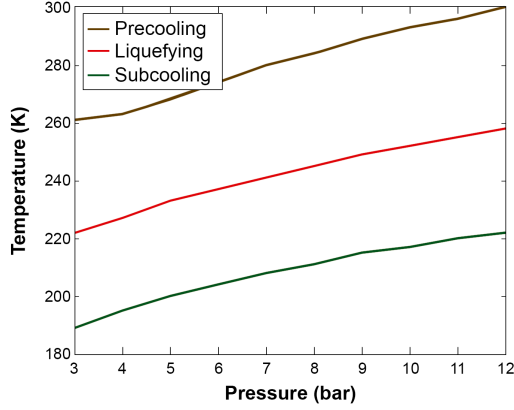
Fig. 3. Minimum pressure of each cycle. The y-axis represents the minimum temperature of the cycle when it enters its respective heat exchanger, and the x-axis represents the minimum pressure provided by the compressor.
