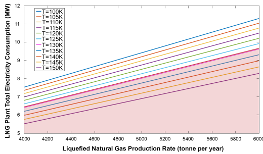
Fig. 5. Influence of the LNG production rate in the available power for different product temperatures. The LNG in this simulation has a 90% mol methane. The operation points have to be above the red zone
