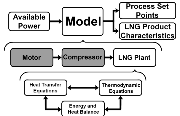
Fig. 1. The model is designed in such a way that it can tell the user to establish a series of set points according to the available power in the plant.
