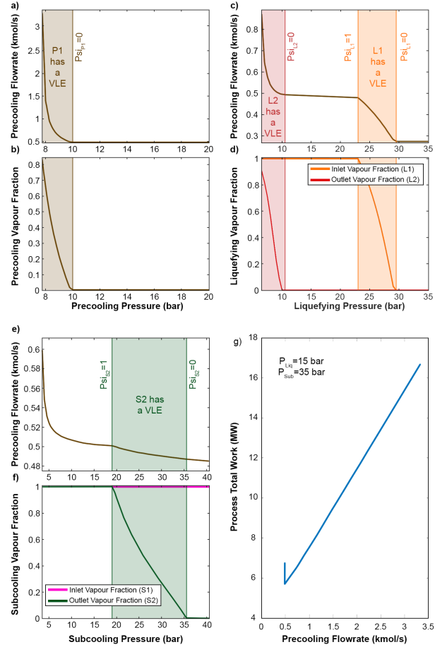
Fig. 4. Influence of the pressure in the precooling cycle flowrate. a) , c) , and e) indicate the flowrate when, respectively, the precooling, the liquefying, and the subcooling pressures vary. b) , d) , and f) show the phases of P_1 , L_1 and S_1 (Inlet), and L_2 and S_2 (Outlet) as a function of the pressure.
