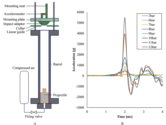
Figure 6 (A) Schematic of the Rig for in vivo Underbody Loading (RivUL). (B) Vertical acceleration of the RivUL seat over time in response to changing pressure input.
