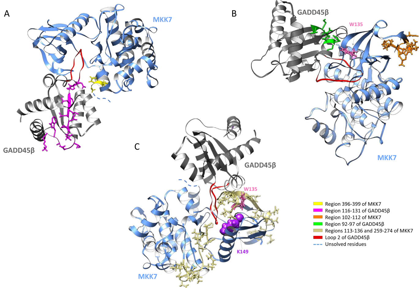
Fig. 5. Ribbon representation of the GADD45 \beta /MKK7 complex in which GADD45 \beta is depicted in grey and MKK7 in blue. (A) Regions 396–399 of MKK7 (yellow) (MKK residues from 400 to 405 cannot be represented because their coordinates have not been solved) and 116–131 of GADD45 \beta (magenta) are represented in stick; (B) residues 102–112 of MKK7 are coloured in orange while residues 92–97 of GADD45 \beta are reported in green. In (C) the MKK7 regions (113–136 and 259–274) cross-linked by the photoactivatable SDA-DTP3 are reported in gold. In all figures the loop 2 of GADD45 \beta is reported in red. In (B) and (C), W135 is highlighted in pink and atoms of K149, responsible of ATP binding, are reported as spheres.
