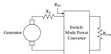
Fig. 5: Using a power converter to get optimal power transfer from the generator
