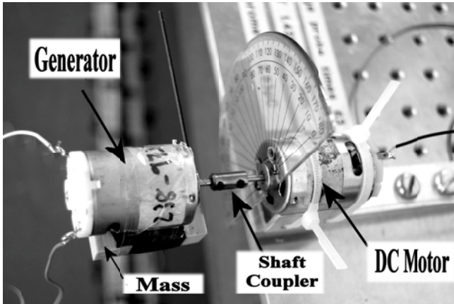
Fig. 2: Experimental setup of the generator and rotational source
