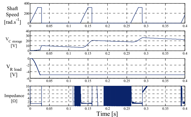
Fig. 7: SPICE simulation results for the model in Fig. 10 with R_{Load} = 10k\Omega and R_A = 1.1\Omega
