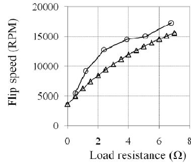
Fig. 4: Flip-over speed vs. load resistances when R_A = 1.1\Omega : experimental (circles) and modelled (triangles)
