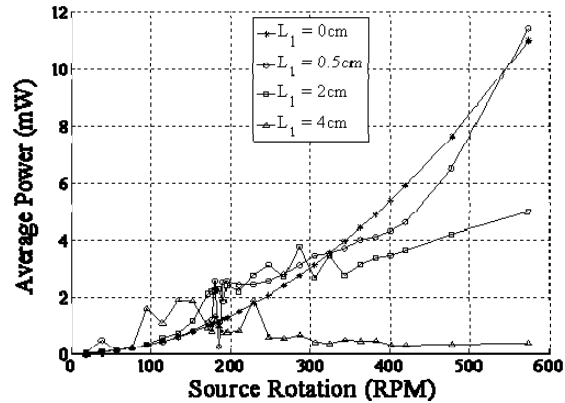
Fig. 9: Average power generated against source rotation at various offset distances, l_1
