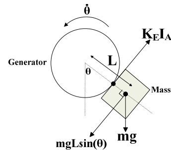
Fig. 1: Schematic of the gravitational torque generator. I_A is the armature current and K_E is the motor constant.
