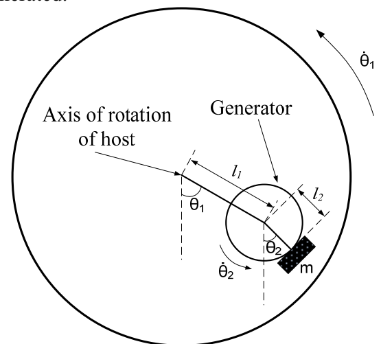
Fig. 8: Schematic of the off-axis generator
