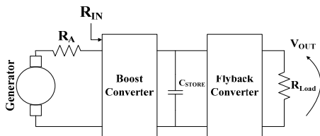
Fig. 6: Using power converters for impedance matching and output voltage regulation
