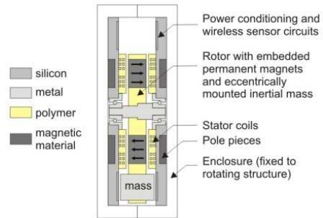
Fig. 10: Schematic of possible microgenerator implementation
