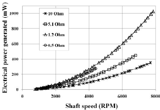
Fig. 3: Measured powers for the specified load resistances when R_A = 1.1\Omega
