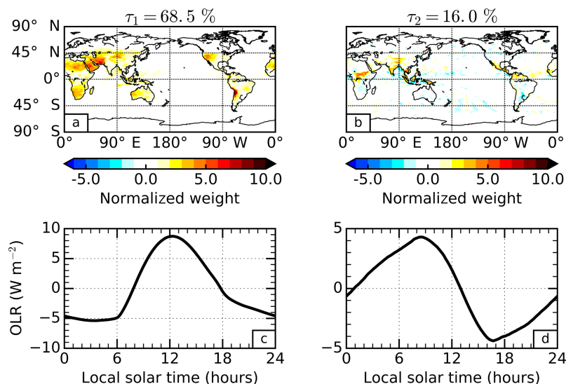
Figure 1. Principal component analysis of the global outgoing long-wave radiation (OLR) diurnal cycle for September 2010 in the Met Office model. The empirical orthogonal functions ( a and b ) and principal components ( c and d ) are presented for the first ( a and c ) and second ( b and d ) most dominant patterns of variability. The percentage variance explained by each pattern is stated above the corresponding empirical orthogonal function.
