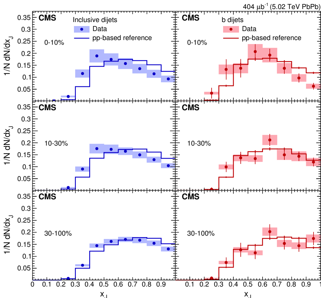
Figure 5. Distributions of x_J in PbPb collisions for inclusive dijets (left) and b dijets (right). Systematic uncertainties are shown as shaded boxes, while statistical uncertainties are shown as vertical lines. The top, middle and bottom rows show the 0–10, 10–30 and 30–100% centrality selections, respectively. The data are compared to a reference obtained by smearing pp according to the jet resolution for the given centrality class, as described in the text.
