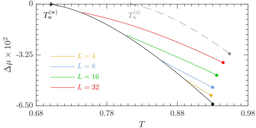
Figure 2. Surface phase diagrams for fluid adsorption near a solvophobic stripe for different stripe width L . Pre-wetting lines for uniform (w)-wall (solid black) and (s)-wall (dashed grey) remain there for all L and are shown together with the unbending lines, the locations of which are different for different L . The pre-wetting lines approach the bulk coexistence line \Delta\mu = 0 tangentially and similarly, each unbending line merges with the pre-wetting line tangentially. The respective temperatures T^* at which the lines merge occur at T^* \approx 0.89, 0.86, 0.81 and 0.75 and approach the pre-wetting critical point as the width decreases.
