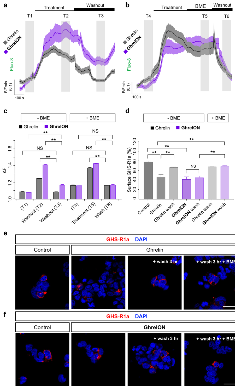
Figure 6. Ghre1ON reversibly activates and internalizes the GHS-R1a. (a) Both ghrelin and Ghre1ON induce large increases in intracellular \text{Ca}^{2+} concentrations in YFP-AD293-SNAP_GHS-R1a, although washout of ligand only restores baseline \text{Ca}^{2+} levels for ghrelin (mean \pm SEM traces shown) (gray shaded area T1–T3 = analysis time window) ( n = 27 –54 cells). (b) Application of beta -mercaptoethanol (BME) for 5 min immediately prior to washout reduces \text{Ca}^{2+} responses to Ghre1ON to baseline levels (mean \pm SEM traces shown) (gray shaded area T4–T6 = analysis time window) ( n = 27 –54 cells). (c) Bar graph showing amplitude of \text{Ca}^{2+} responses to ghrelin and Ghre1ON before and after washout \pm BME ( n = 27 –54 cells) (T1–T6 relate to time windows shown in a and b). (d) Treatment of YFP-AD293-SNAP_GHS-R1a cells with ghrelin for 1 h leads to GHS-R1a internalization, which can be partially reversed following washout and incubation for a further 3 h. Ghre1ON exerts similar effects, but these can only be washed out following prior application of BME for 10 min ( n = 10 –12 images from two experiments). (e) Representative images showing that ghrelin reduces surface GHS-R1a expression (detected via the FLAG-tag), which is reversed by a wash step (scale bar = 33 \mu\text{m} ). (f) As for (e), but showing that plasma membrane GHS-R1a recycling can only be achieved by application of BME to Ghre1ON-treated YFP-AD293-SNAP_GHS-R1a cells. **P < 0.01 and NS, nonsignificant, as indicated; Student's t test or one-way ANOVA (with Bonferroni's posthoc test). Ghrelin and Ghre1ON were applied at 100 nM and 800 nM, respectively. BME was applied at 10 mM. Values are the mean \pm SEM.
