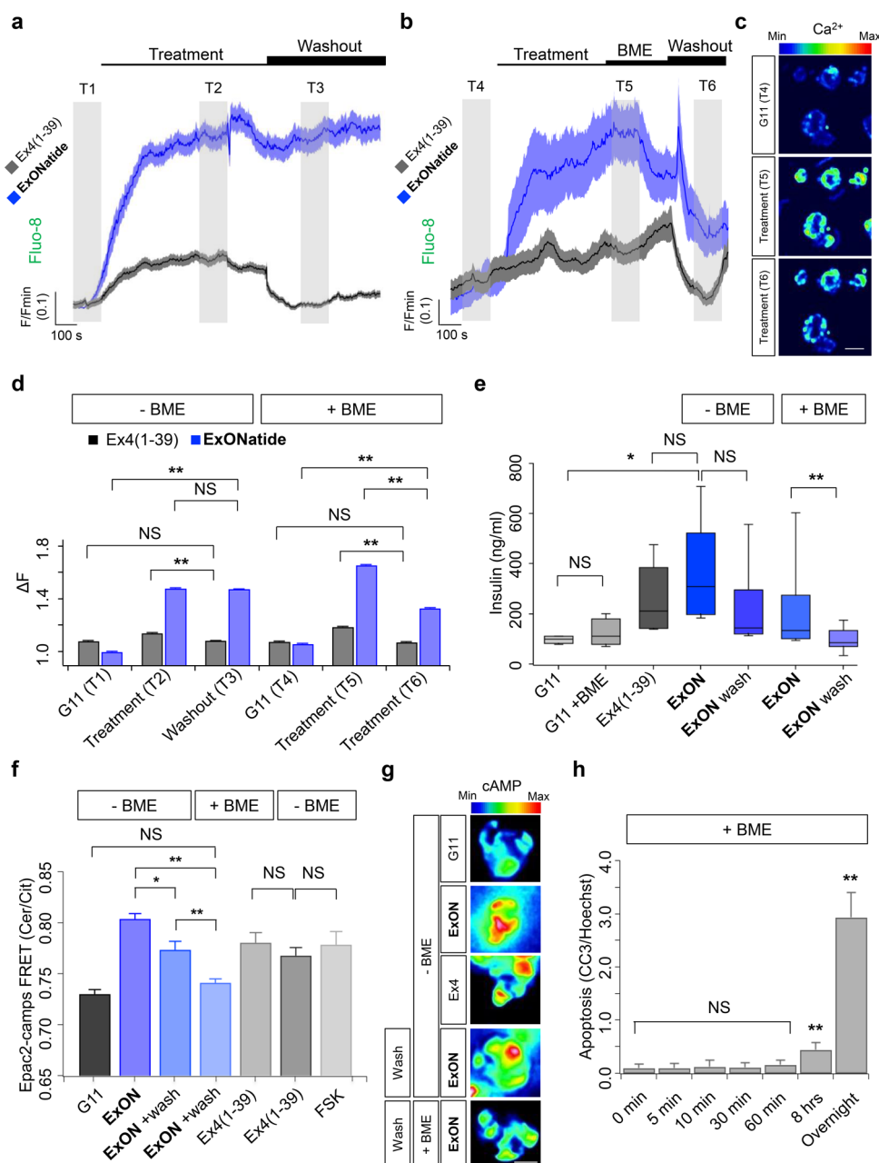
Figure 3. ExONatide leads to prolonged \text{Ca}^{2+} and cAMP signaling. (a) ExONatide induces \text{Ca}^{2+} rises in MIN6B1-SNAP_GLP-1R cells similarly to Ex4(1–39), but this cannot be washed out with buffer (mean \pm SEM traces shown) (gray shaded area T1–T3 = analysis time window) ( n = 29 –34 cells). (b) Application of beta -mercaptoethanol (BME) for 5 min immediately prior to washout allows \text{Ca}^{2+} responses to ExONatide to be subsequently reduced (mean \pm SEM traces shown) (gray shaded area T4–T6 = analysis time window) ( n = 34 cells). (c) Representative images showing \text{Ca}^{2+} responses to ExONatide in MIN6B1-SNAP_GLP-1R cells before (T4), during (T5) and after (T6) application of BME. (d) Bar graph showing amplitude of \text{Ca}^{2+} responses to Ex4(1–39) and ExONatide before and after washout \pm BME ( n = 29 –34 cells) (T1–T6 relate to time windows shown in a and b). (e) Box and whiskers plot showing that ExONatide-stimulated insulin secretion can only be washed out following application of BME ( n = 8 wells) (Ex4(1–39)-alone was used as a positive control) (G11; 11 mM glucose). (f) As for (a), but FRET assays for intracellular cAMP 15 min following application of ligand or washout ( n = 40 –71 cells). (g) Representative images showing FRET responses to ExONatide in MIN6B1-SNAP_GLP-1R cells before and after application of BME. (h) BME was unable to significantly induce apoptosis over 60 min, as determined using immunostaining for cleaved caspase 3 (CC3) (overnight incubation serves as the positive control) ( n = 3 experiments). ** P < 0.01 and NS, nonsignificant, as indicated or vs control; Student's t test, one-way ANOVA (with Bonferroni's or Tukey's posthoc test) or Kruskal–Wallis test (with Dunn's multiple comparison test). ExONatide and Ex4(1–39) were applied at 800 nM and 10 nM, respectively. BME was applied at 10 mM. Values are the mean \pm SEM unless otherwise stated.
