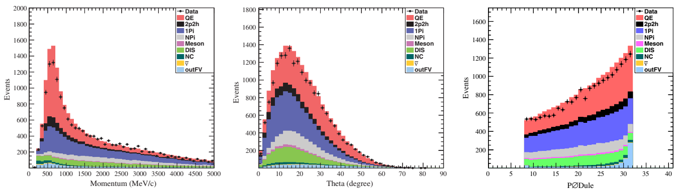
FIG. 3. FHC beam CCINC \nu_\mu event candidate distributions of the \mu^- momentum in MeV/c (left), the muon \theta_\mu angle in degrees (middle), and interaction vertex position by P \emptyset Dule (right). Note backgrounds in the CCINC sample are the NC (dark green), \bar{\nu}_\mu induced events (yellow) and the out of fiducial volume events (light blue). There are negligible \bar{\nu}_\mu backgrounds (yellow) in the FHC sample.
