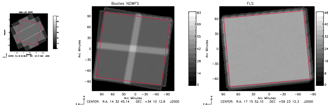
Figure 5. Maps of the number of bolometer samples per pixel in SPIRE 250 \mu\text{m} blank field observations from Level 6. From the left they are XMM-LSS-SWIRE (#39), Boötes NWDFS (#37) taken early with conservative overlap) and FLS (#40, from SDP). All are parallel mode observations with a nominal coverage of two scans. Overlaps produce a maximum coverage of four scans in XMM-LSS-SWIRE and eight in Boötes.
