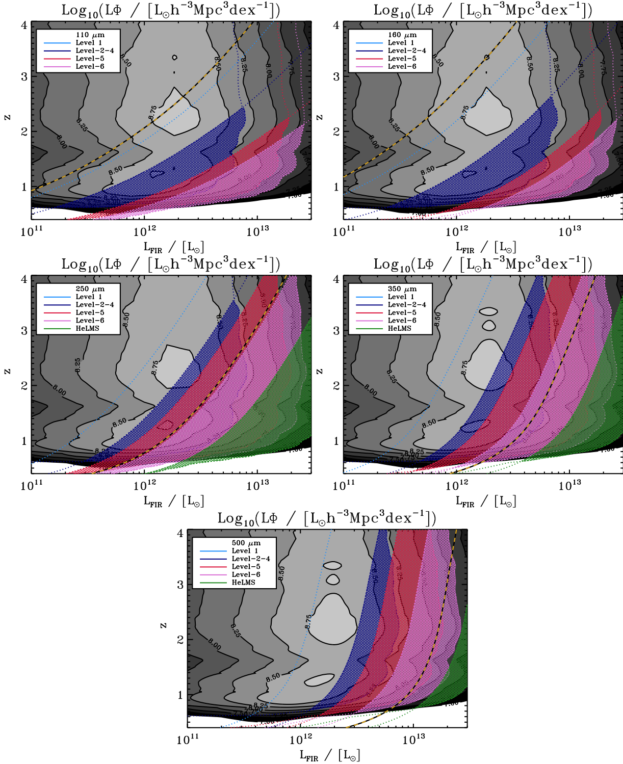
Figure 2. Far infrared luminosity density in \log_{10}(L_{\odot}h^{-3}\text{Mpc}^3\text{dex}^{-1}) (grey-scale and contour diagram) as a function of far infrared luminosity ( x -axis) and redshift ( y -axis) – from the model of Lagache et al. 2003. The power of different survey elements to probe this space are indicated by overlays. Each panel shows survey elements at different wavelengths; reading left-to-right from the top they are 100, 160, 250, 350 and 500 \mu\text{m} . Surveys are deemed to properly sample the space if they can detect galaxies of these FIR luminosities at the 5- \sigma instrumental noise level and with more than 75 galaxies in bins of \Delta \log L \Delta z = 0.1 . These two constraints are marked with dotted lines and are hatched. The different survey levels defined in Table 7 are shown with: Levels 2-4 – blue; Level 5 – red; Level 6 – magenta and HeLMS – green. Level-1 (cyan) does not have enough volume to satisfy the number of galaxies criterion and so only the instrumental noise limit is shown. The 5 \sigma confusion noise levels (after 5 \sigma clipping) from Berta et al. (2011, at 100 and 160 \mu\text{m} ) and Nguyen et al. (2010, at 250, 350 and 500 \mu\text{m} ) with yellow/black lines. Note the bimodal peaks at z \sim 1 and z \sim 2.5
