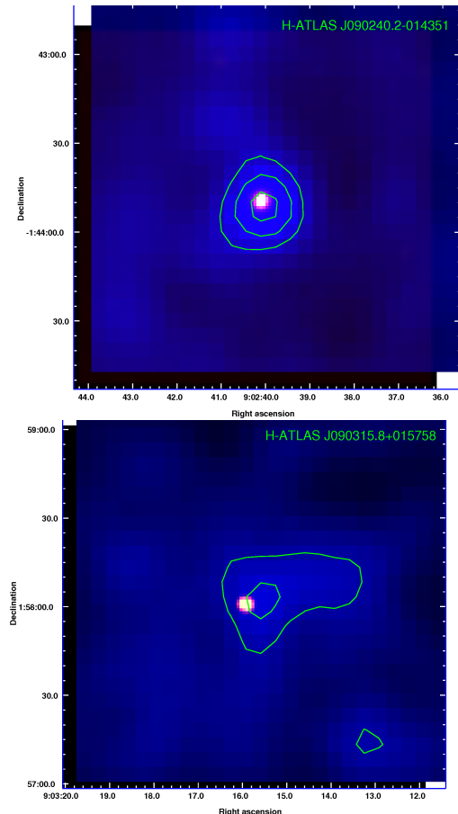
Fig. 3. Three colour images of the two candidate debris disks detected by H-ATLAS. Red & green channels are 2MASS J & K_s respectively. The blue channel is SPIRE 250 \mu\text{m} , smoothed by a 3 pixel Gaussian kernel to increase the signal to noise ratio. Contours are of 250 \mu\text{m} emission starting at 3\sigma and spaced by 2\sigma .
