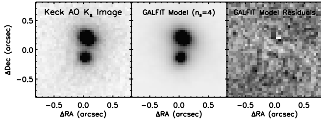
Figure 2. GALFIT modeling of G15v2.779. Left: Keck AO K_S -band image (as in Figure 1). Middle: best-fit GALFIT model (assuming n_s = 4 for both lensing galaxies). Right: residuals obtained after subtracting the best-fit model from the Keck data. Both morphologies are consistent with early-type galaxies.
