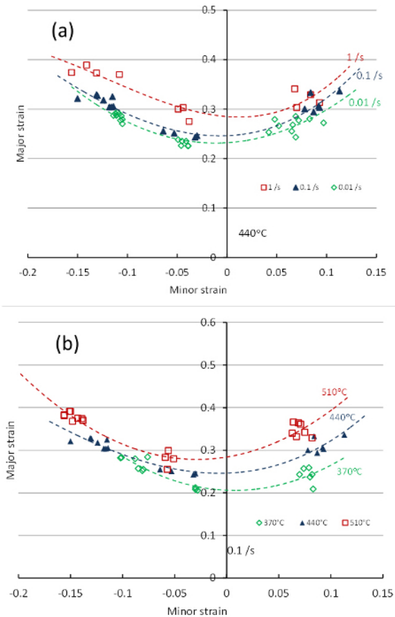
Figure 4: FLDs of AA6082 at (a) different strain rates and (b) different temperatures under hot stamping conditions. The symbols are the results of the forming limits under different conditions. The dashed lines were obtained through the polynomial fitting algorithm. Please click here to view a larger version of this figure.
