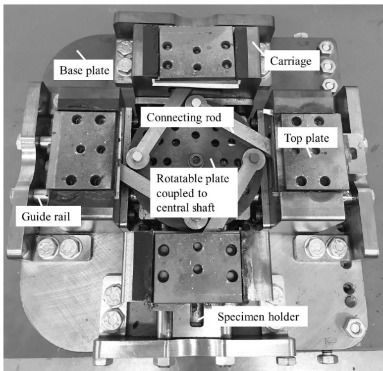
Figure 2: The assembled biaxial testing apparatus. The apparatus includes a base plate, a central shaft, rotatable plates, carriages, guide rails, and connecting rods. It is mounted in the chamber of the resistance heating uniaxial testing machine. Key components have been marked in the figure. Please click here to view a larger version of this figure.
