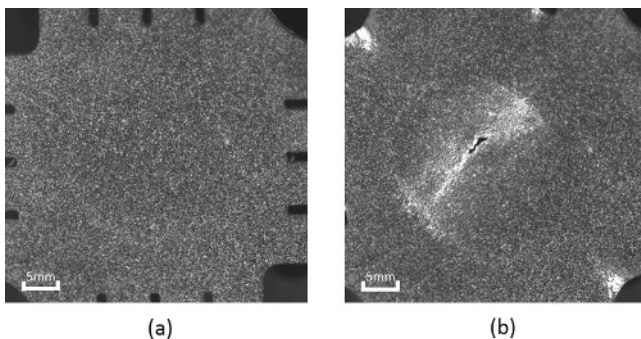
Figure 1: An example of a stochastic pattern in a cruciform specimen before biaxial stretching (a) and after biaxial stretching (b). The pattern with white dots on a black background is captured by the high-speed camera during tests. The size and density of the speckles within a pattern are subjected to the standard requirements of DIC analysis 15 . Please click here to view a larger version of this figure.
