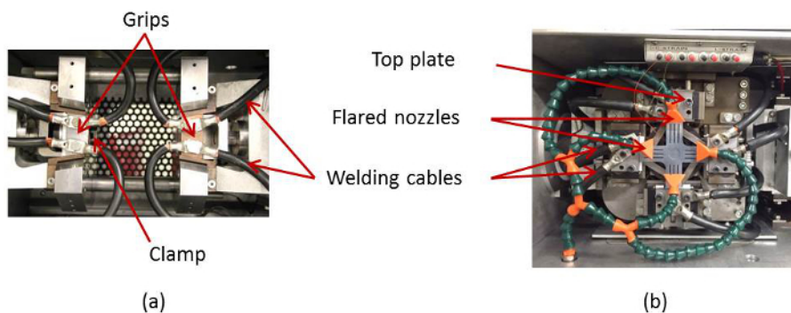
Figure 3: Setup of grips and the biaxial testing apparatus in the chamber of the uniaxial testing machine. (a) The grips and the clamp. (b) The biaxial testing apparatus and nozzles for air cooling. Please click here to view a larger version of this figure.
