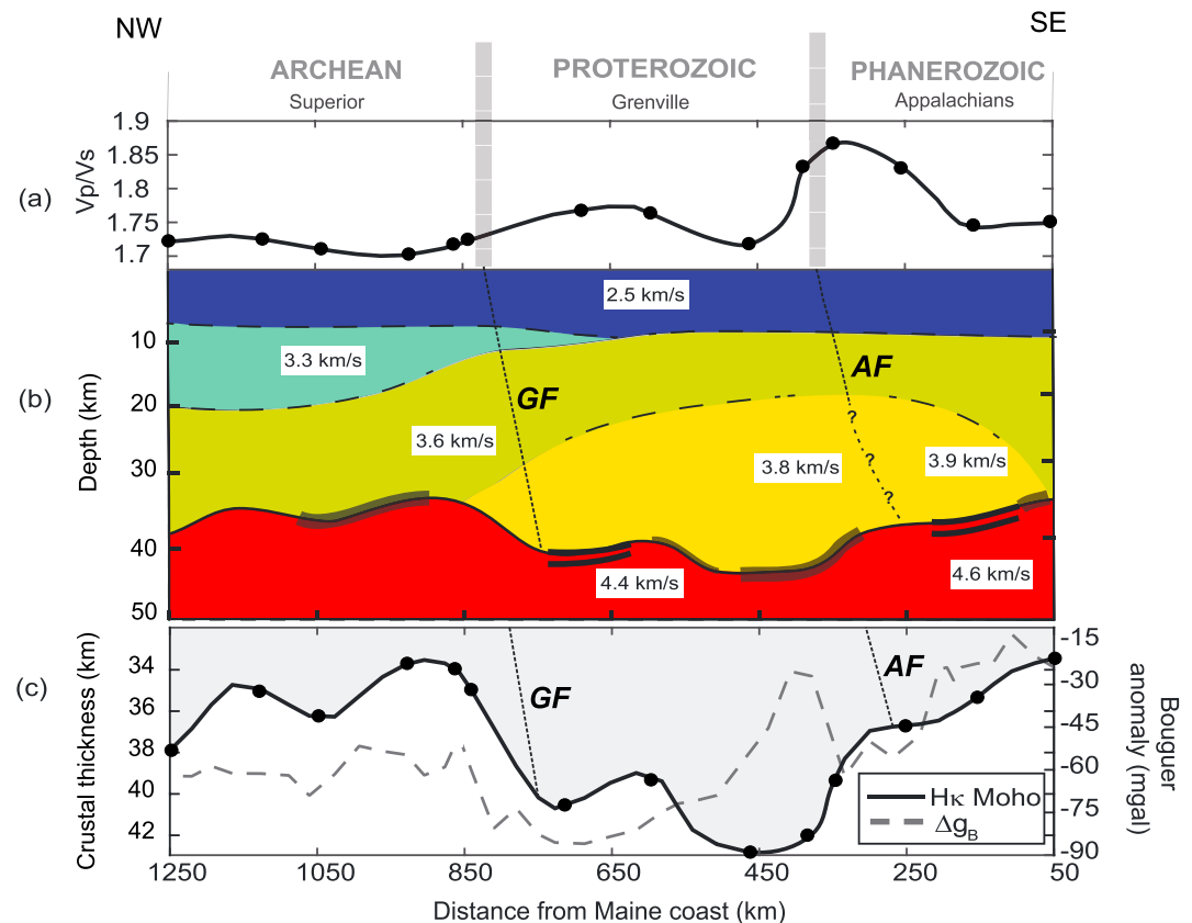
Figure 8. Structure along the QM-III NW-SE profile, based on receiver function modeling. (a) V_p/V_s ratios from H-\kappa stacking. (b) Shear wave velocity profile based on Bayesian inversion, interpolated between individual stations. Thick semitransparent lines indicate regions with a gradational Moho; double lines indicate a doubled Moho discontinuity. (c) Crustal thickness and Bouguer gravity anomaly. GF: Grenville Front and AF: Appalachian Front.
