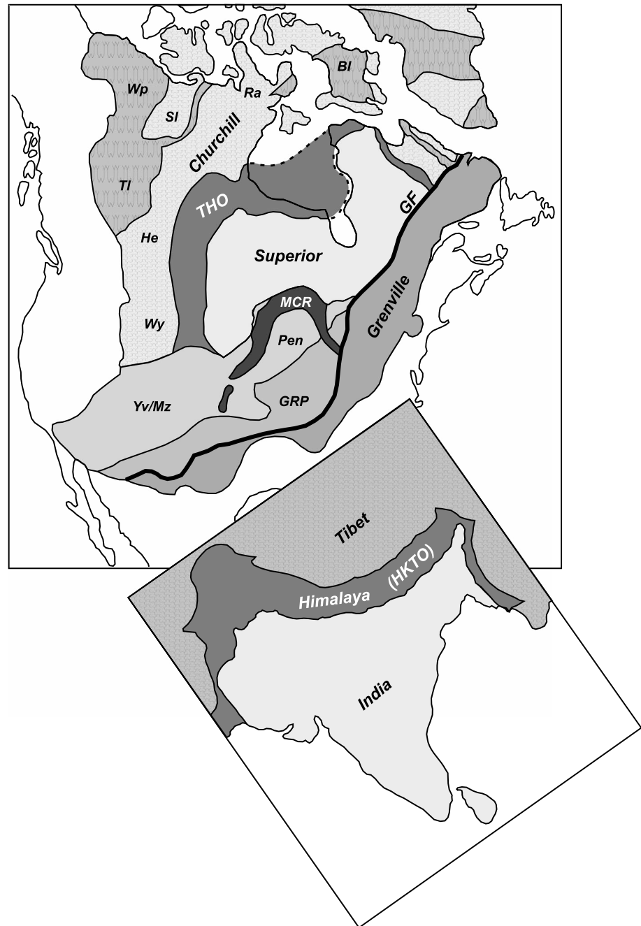
Figure 14. Simplified tectonic maps of (top) North America and the (bottom) India-Asia collision. The upper plate of the THO and HKTO collisions is shown with textured shading, and the lower plate is shown in uniform shade(s) of gray. Abbreviations: Archean domains: He: Hearne; Ra: Rae; Wy: Wyoming; Sl: Slave. Paleoproterozoic domains: THO: Trans-Hudson Orogen; Wp: Wopmay; TI: Taltson; BI: Baffin Island; Yv/Mz: Yavapai/Mazatzal; Pen: Penokean. Mesoproterozoic domains: GRP: Granite-Rhyolite Province; MCR: Mid-continent Rift; GF: Grenville Front. Modified from Hoffman [1989], Rivers [2015], St-Onge et al. [2006], and Weller and St-Onge [2017].
