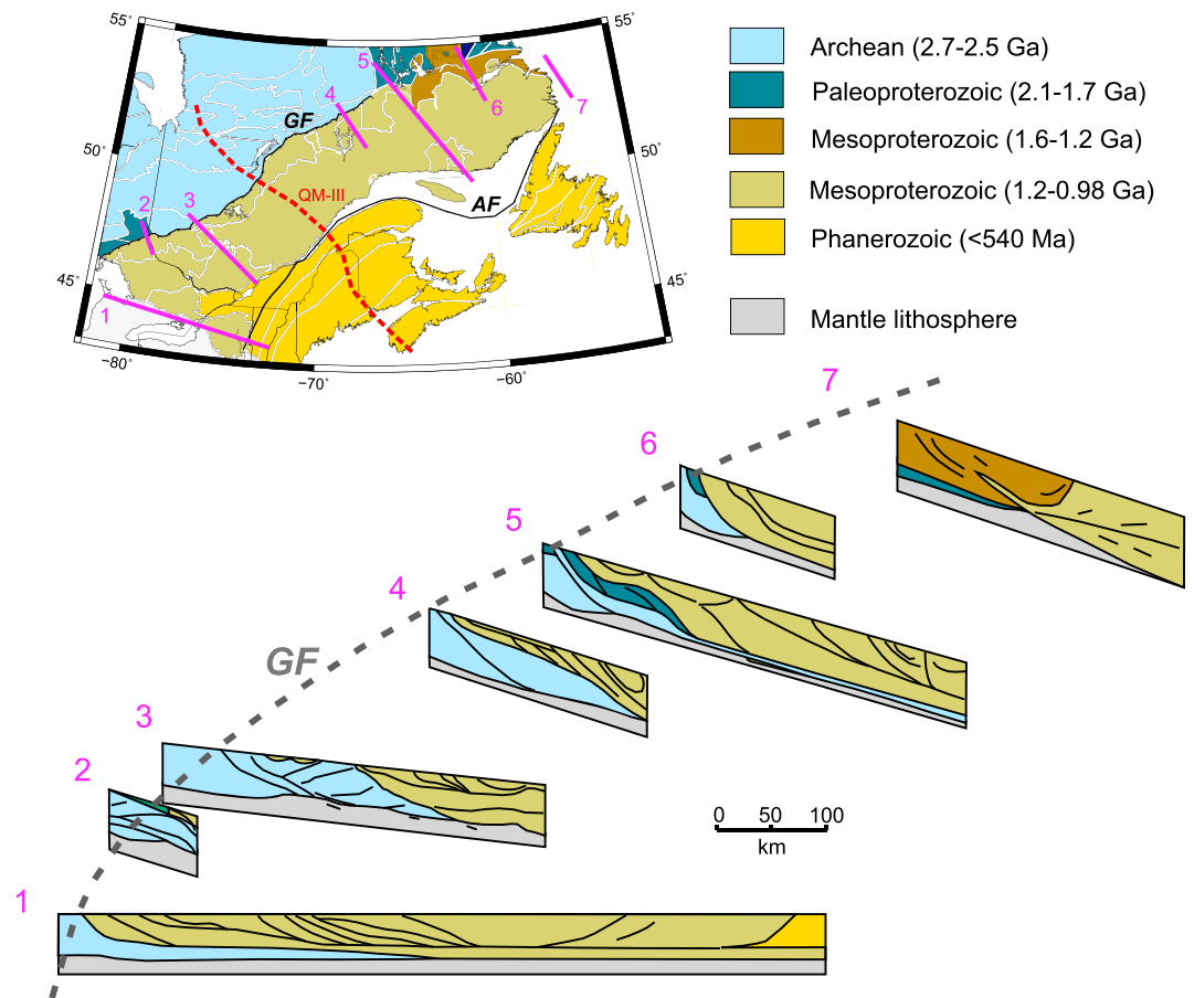
Figure 7. Crustal cross sections for the Grenville Province based on LITHOPROBE seismic reflection/refraction data. GF: Grenville Front. Modified from Hammer et al. [2010]. The QM-III transect (2012–2015) of broadband seismograph stations is also shown.
