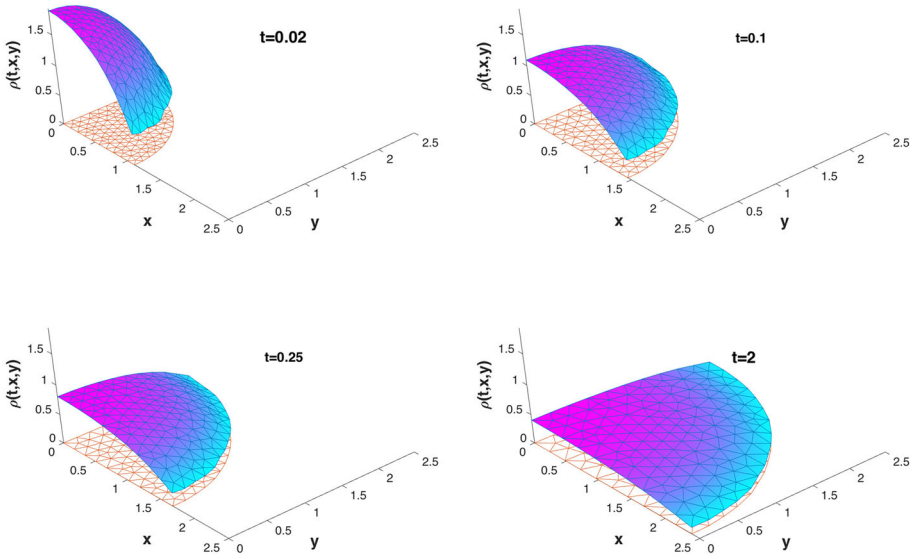
Fig. 2 Numerical experiment 1: fully discrete evolution of our approximation for the self-similar solution to the free porous medium equation. Snapshots are taken at times t = 0.02, t = 0.1, t = 0.25, and t = 2.0
