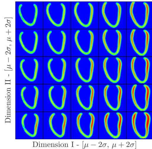
Fig. 9: Anatomical variations captured by the latent representations in T-L network (swipe from \mu - 2\sigma to \mu + 2\sigma ). Based on our observation, the first and second dimensions capture the variation in the wall thickness of the myocardium (x-axis) and lateral wall of the ventricle (y-axis).
