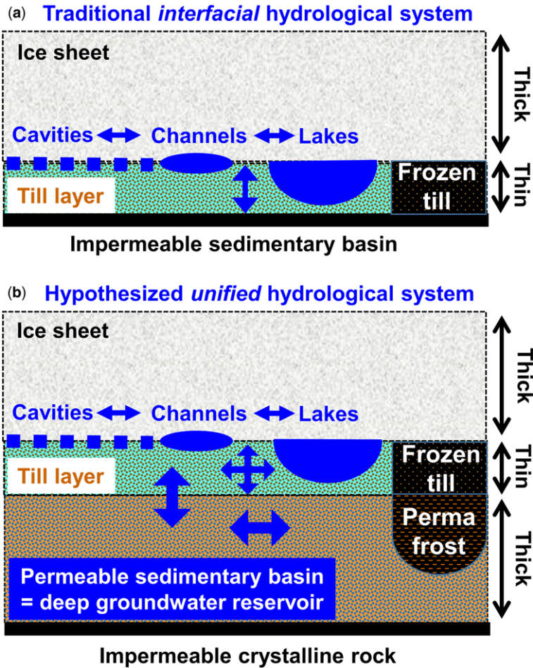
Fig. 1. (a) Interfacial subglacial water system of interconnected till, linked-cavities, channels, lakes and areas of basal freezing, considered in ice-sheet models so far (e.g. Fig. 3). (b) Unified subglacial water system, where the interfacial system exchanges water with a deep groundwater reservoir. The thick arrows are the main water-flow directions. An extra four hydrological processes arise in unified (b) compared to interfacial (a) systems, which must be evaluated by models (not to scale; ice and the sedimentary basin are often kilometres thick, the till layer is metres thick).
