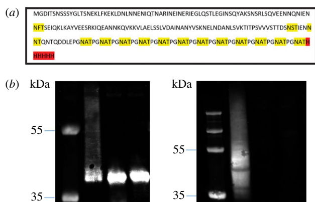
Figure 8. Glycosylation of engineered acceptor protein (JC1) by NGT and \alpha 6GlcT. (a) Amino acid sequence of the new target glycoprotein JC1. Highlighted in yellow are glycosylation sequons, and in red, the hexa-HIS tag used for protein purification. (b) Glycosylation of the acceptor protein JC1 with NGT and \alpha 6GlcT. Left panel: anti-histidine tag western blot; right panel, anti-dextran western blot. Lane 1: JC1 expressed with functional NGT and \alpha 6GlcT; lane 2: JC1 with NGT K441A and \alpha 6GlcT; lane 3: JC1 with NGT but non-functional \alpha 6GlcT.
