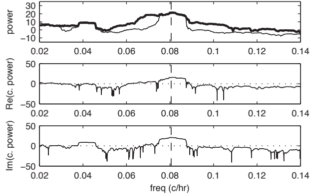
Fig. 3. Upper plot: the spectrum S_Z(f) , in dB, for one of the three current series. Thin line: the counterclockwise (positive) frequencies; thick line: clockwise (negative) frequencies. Middle plot: |\text{Re}\{R_Z(f)\}| on 10 \log_{10} scale. Lower plot: |\text{Im}\{R_Z(f)\}| on 10 \log_{10} scale. The dashed line marks the semi-diurnal tidal frequency.
