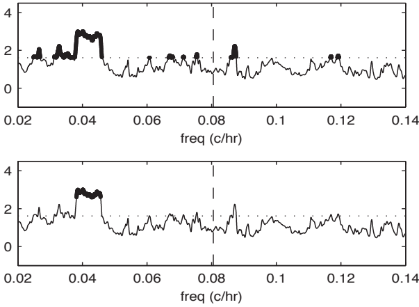
Fig. 4. The test statistic M(f) (solid) and the critical value (dotted line) for \alpha = 0.05 for the frequency-specific propriety test for the vector \mathbf{Z}_t = [Z_{1,t}, Z_{2,t}, Z_{3,t}]^T . Upper: test at individual frequencies; rejection occurs at all frequencies where M(f) exceeds the critical value, such frequencies being marked by heavy dots. Lower: overall test results using FDRd with \alpha = 0.05 . Frequencies causing rejection are again marked by heavy dots. The dashed line marks the semi-diurnal tidal frequency.
