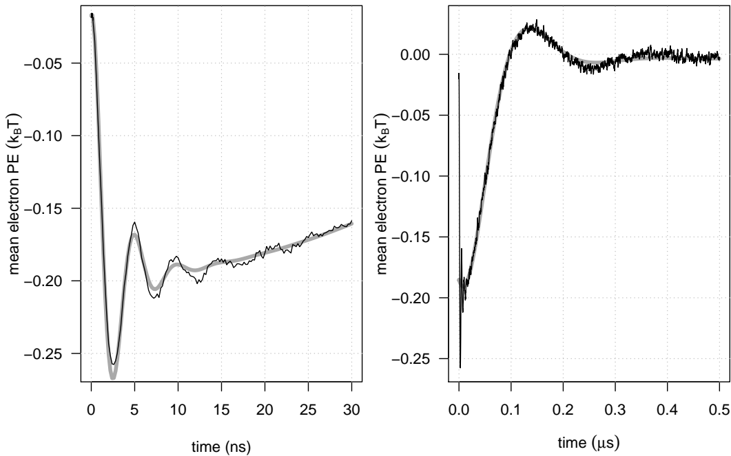
Figure 3. The time evolution of mean electron potential energy for a pot simulation with non-equilibrium initial state. Oscillations are seen on the short timescale of electron plasma oscillations (left) and on the longer timescale of ion plasma oscillations (right). The overlaid non-linear oscillation curves, from equation (6) with the least-squares-fitted parameters shown in table 2, are shown as thick grey lines.
