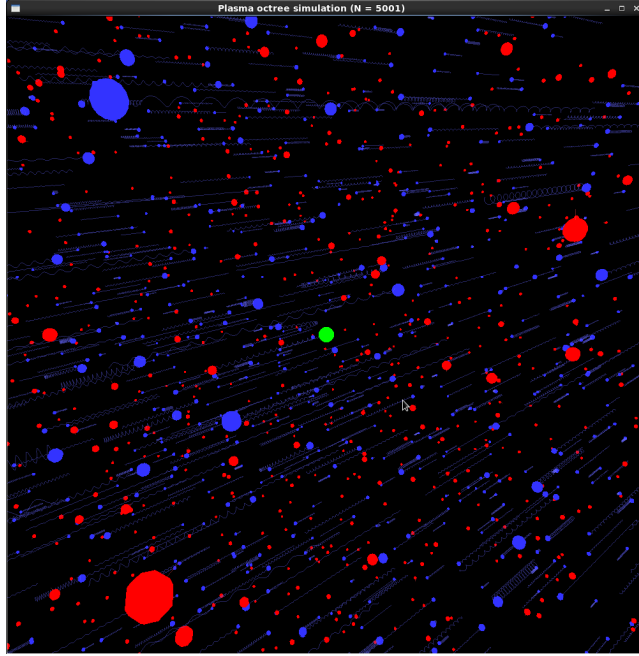
Figure 1. An example of pot 's graphical user interface (GUI) for a simulation containing 2500 (blue) electrons, 2500 (red) ions and a single (green) dust grain with an applied magnetic field of 1 T; full-scale simulations have been performed with 150000 particles in total. The particles' helical trajectories and the dust grain are shown to scale while the ions and electrons, being microscopic and invisible on this scale, are represented by spheres much larger than their physical size. The GUI can be initialized by compiling pot using a flag definable in pot 's source code. It has been particularly useful in testing for sensible particle collection and reinjection and for ensuring steady particle gyro-orbits.
