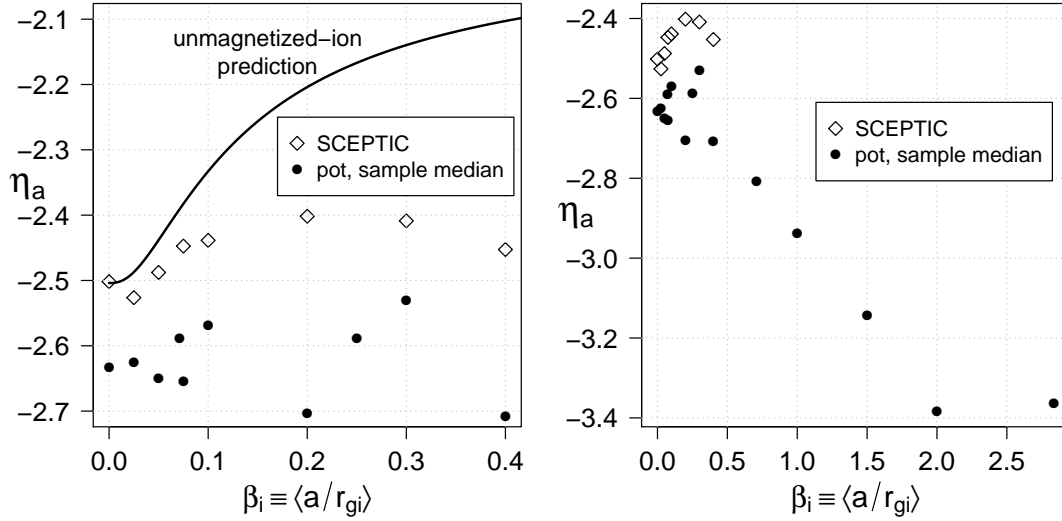
Figure 6. \eta_a as a function of \beta_i , as estimated using: SCEPTIC [27], median equilibrium values in pot runs, and the assumption that ions remain unmagnetized [12]. pot 's results support rejection of the unmagnetized-ion hypothesis. pot does not assume the Boltzmann relation for electrons, so its results can be reliably extended to high magnetic field strengths.
