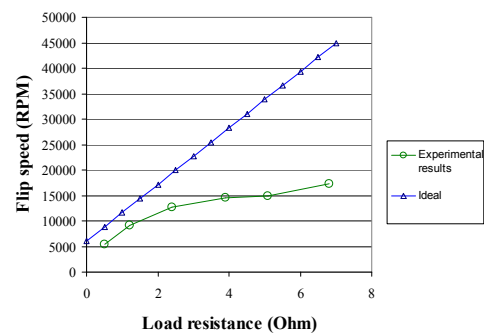
Figure 5. Speed at which the angle of deflection exceeds 90^\circ ; for armature resistance of 1.1 \Omega .
