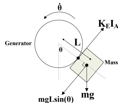
Figure 2. Torque due to the generator and mass.
