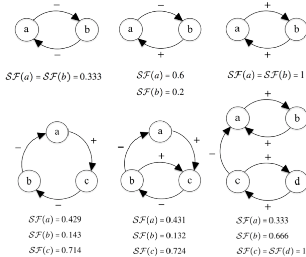
Figure 1. Example BAFs with strengths of arguments as indicated
